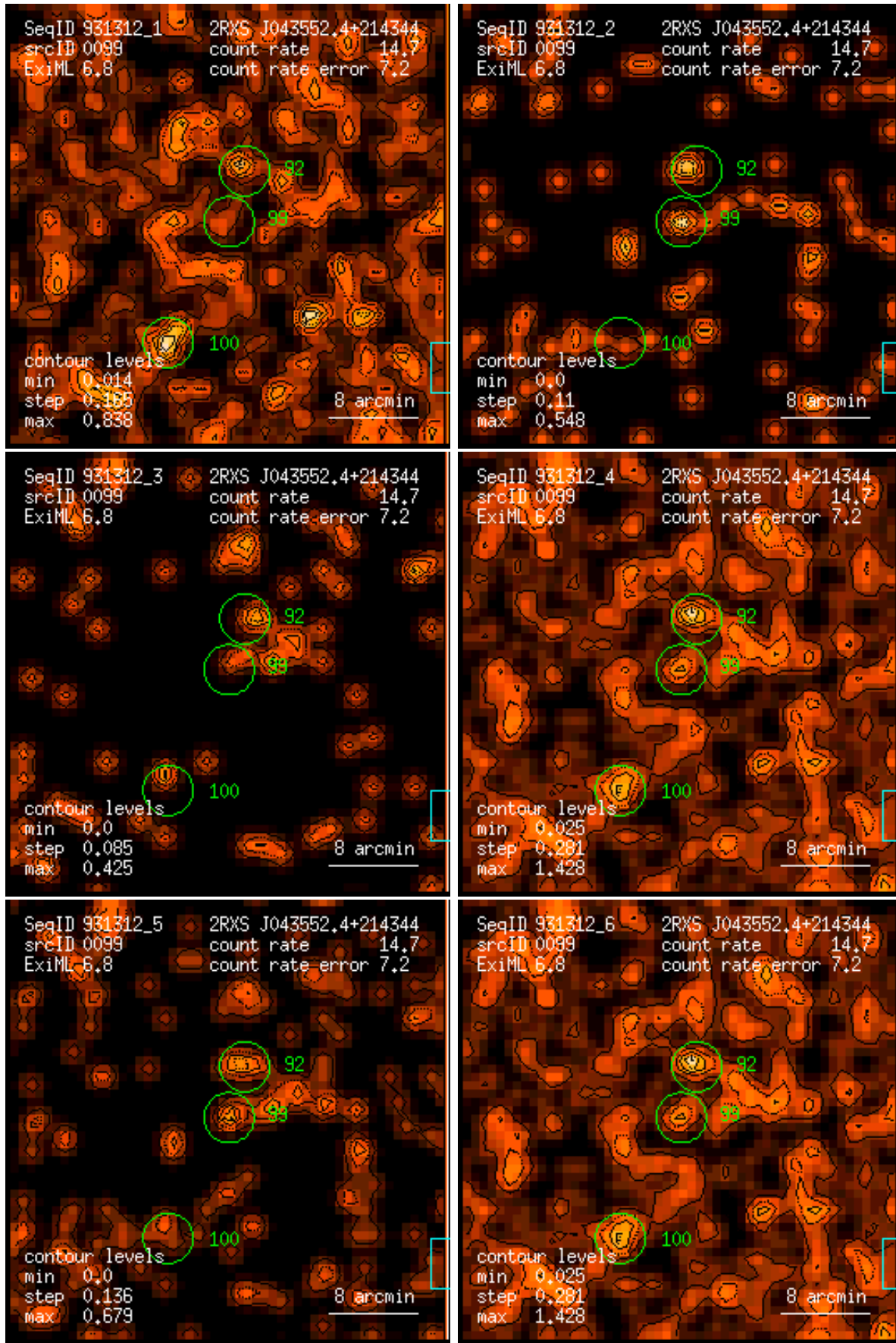
Figure 99: RASS 931312: detection 0099: band rate images, Gaussian filter: (1) PSPC channels 11 – 41, (2) 52 – 90, (3) 91 – 201, (4) 11 – 235, (5) 52 – 201, (6) 11 – 201. Broad band rates in counts/ks. Band rate contour levels in counts/ks/arcmin 2 .
