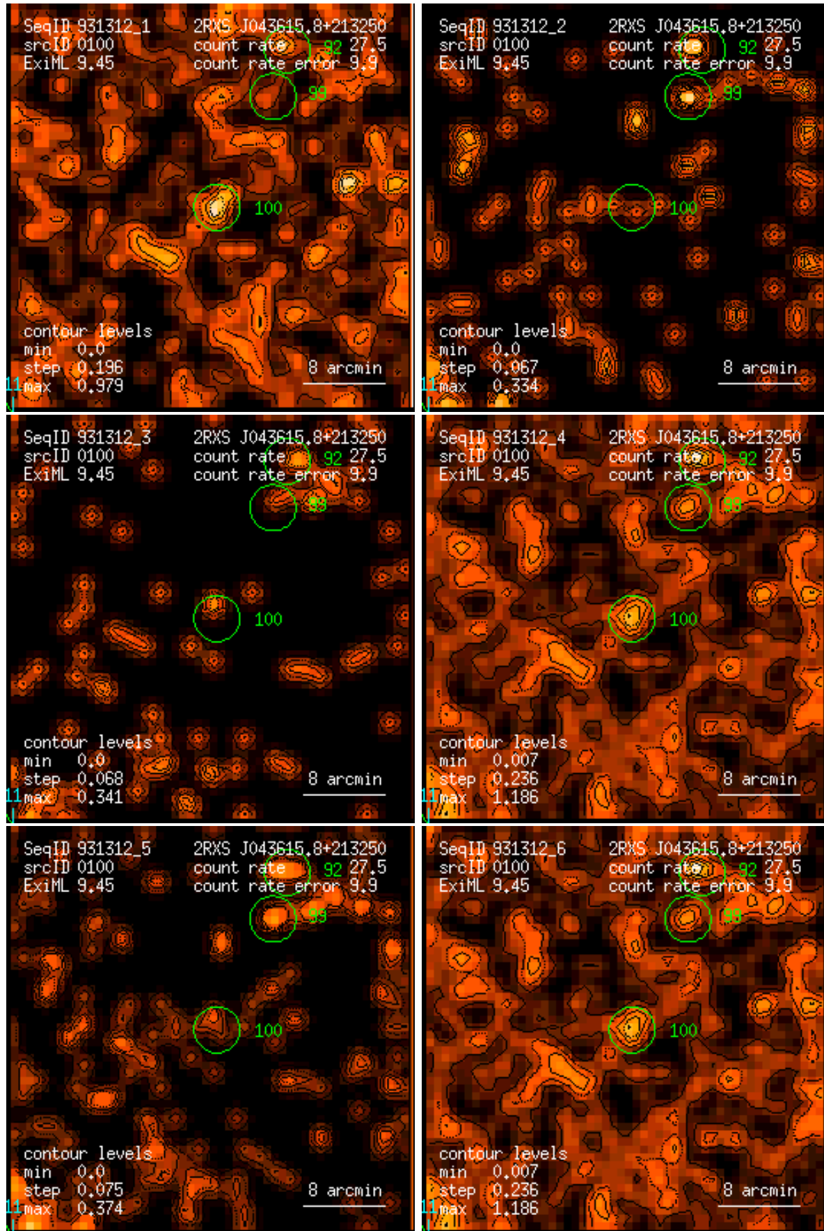
Figure 100: RASS 931312: detection 0100: band rate images, Gaussian filter: (1) PSPC channels 11 – 41, (2) 52 – 90, (3) 91 – 201, (4) 11 – 235, (5) 52 – 201, (6) 11 – 201. Broad band rates in counts/ks. Band rate contour levels in counts/ks/arcmin 2 .
