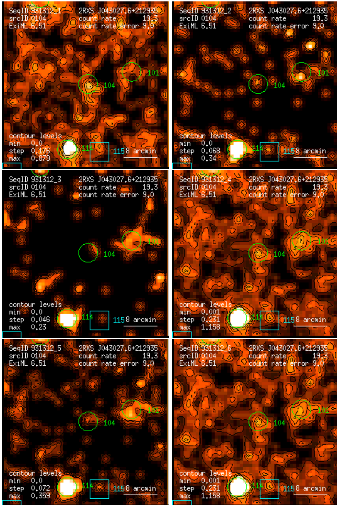
Figure 104: RASS 931312: detection 0104: band rate images, Gaussian filter: (1) PSPC channels 11 – 41, (2) 52 – 90, (3) 91 – 201, (4) 11 – 235, (5) 52 – 201, (6) 11 – 201. Broad band rates in counts/ks. Band rate contour levels in counts/ks/arcmin 2 .
