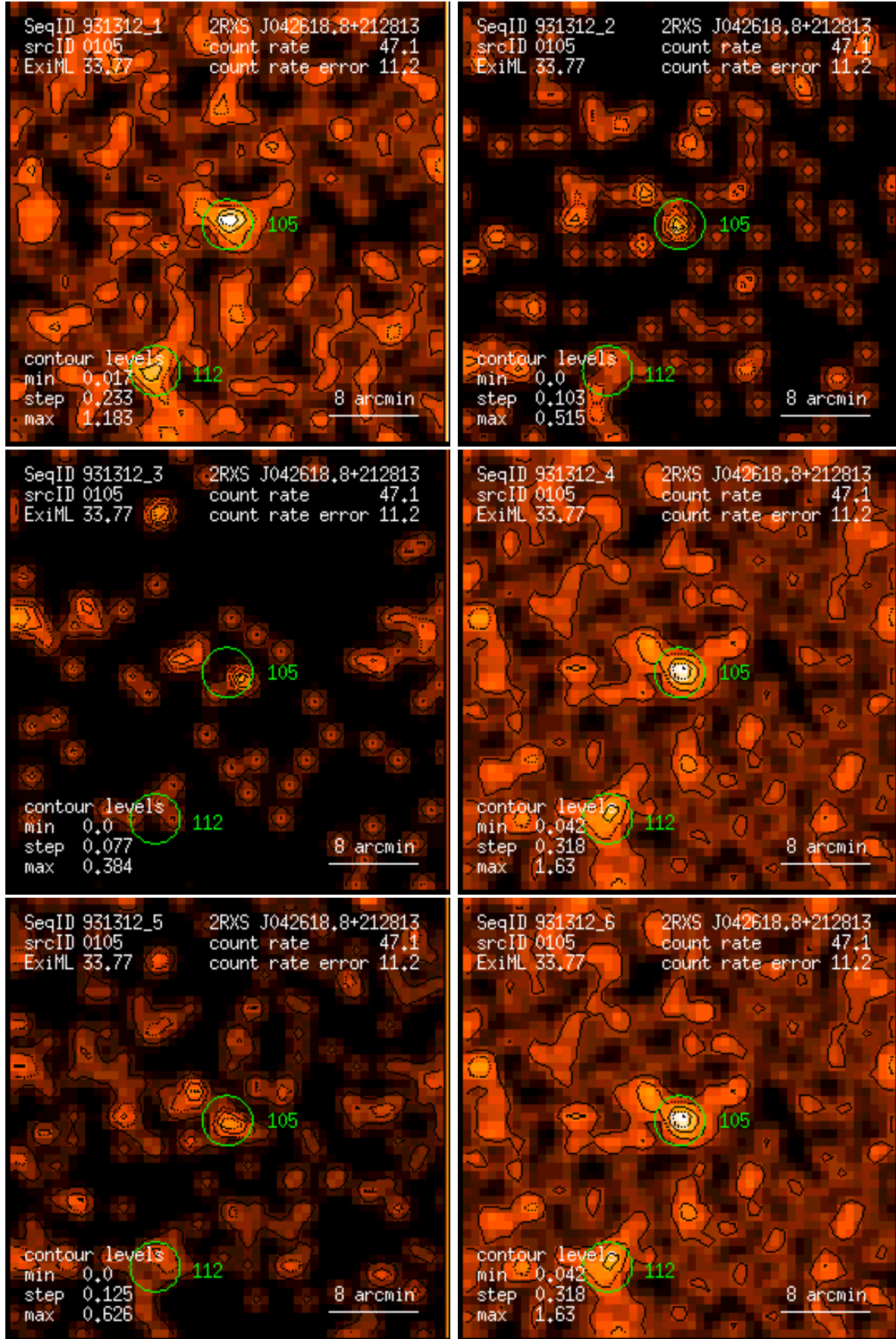
Figure 105: RASS 931312: detection 0105: band rate images, Gaussian filter: (1) PSPC channels 11 – 41, (2) 52 – 90, (3) 91 – 201, (4) 11 – 235, (5) 52 – 201, (6) 11 – 201. Broad band rates in counts/ks. Band rate contour levels in counts/ks/arcmin 2 .
