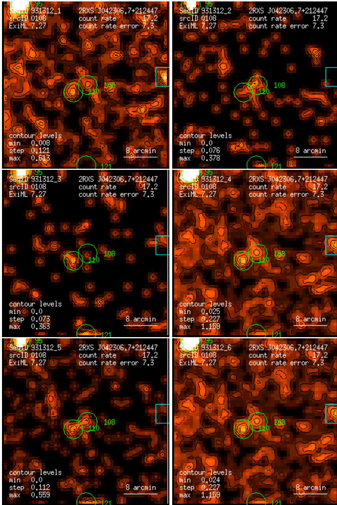
Figure 108: RASS 931312: detection 0108: band rate images, Gaussian filter: (1) PSPC channels 11 – 41, (2) 52 – 90, (3) 91 – 201, (4) 11 – 235, (5) 52 – 201, (6) 11 – 201. Broad band rates in counts/ks. Band rate contour levels in counts/ks/arcmin 2 .
