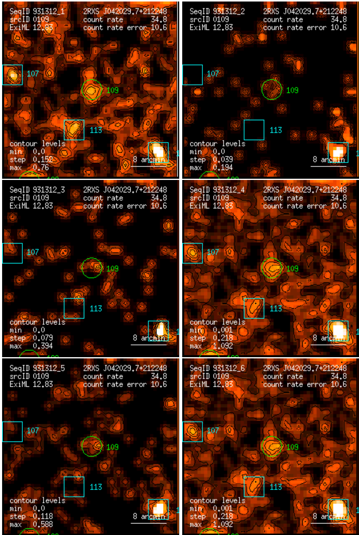
Figure 109: RASS 931312: detection 0109: band rate images, Gaussian filter: (1) PSPC channels 11 – 41, (2) 52 – 90, (3) 91 – 201, (4) 11 – 235, (5) 52 – 201, (6) 11 – 201. Broad band rates in counts/ks. Band rate contour levels in counts/ks/arcmin 2 .
