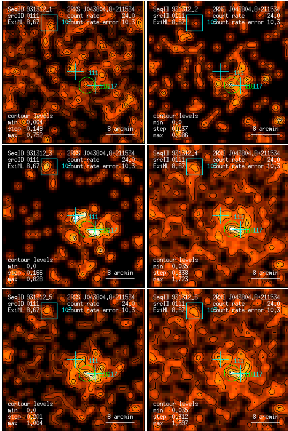
Figure 111: RASS 931312: detection 0111: band rate images, Gaussian filter: (1) PSPC channels 11 – 41, (2) 52 – 90, (3) 91 – 201, (4) 11 – 235, (5) 52 – 201, (6) 11 – 201. Broad band rates in counts/ks. Band rate contour levels in counts/ks/arcmin 2 .
