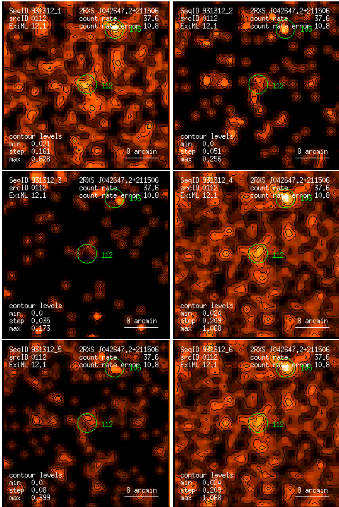
Figure 112: RASS 931312: detection 0112: band rate images, Gaussian filter: (1) PSPC channels 11 – 41, (2) 52 – 90, (3) 91 – 201, (4) 11 – 235, (5) 52 – 201, (6) 11 – 201. Broad band rates in counts/ks. Band rate contour levels in counts/ks/arcmin 2 .
