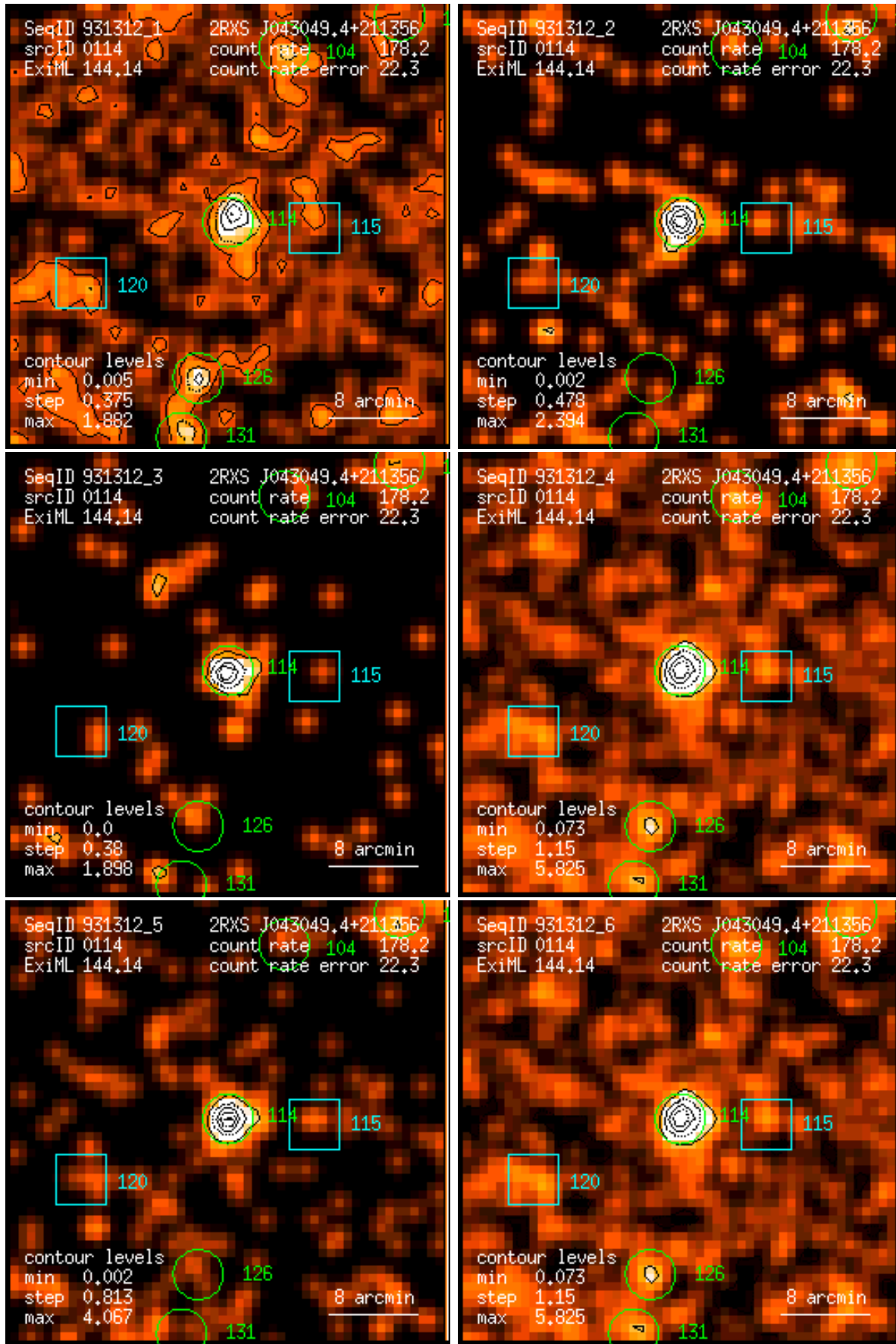
Figure 114: RASS 931312: detection 0114: band rate images, Gaussian filter: (1) PSPC channels 11 – 41, (2) 52 – 90, (3) 91 – 201, (4) 11 – 235, (5) 52 – 201, (6) 11 – 201. Broad band rates in counts/ks. Band rate contour levels in counts/ks/arcmin 2 .
