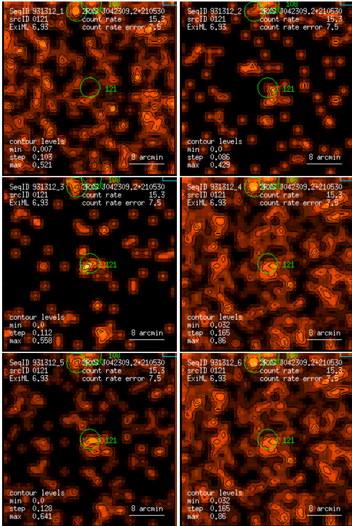
Figure 121: RASS 931312: detection 0121: band rate images, Gaussian filter: (1) PSPC channels 11 – 41, (2) 52 – 90, (3) 91 – 201, (4) 11 – 235, (5) 52 – 201, (6) 11 – 201. Broad band rates in counts/ks. Band rate contour levels in counts/ks/arcmin 2 .
