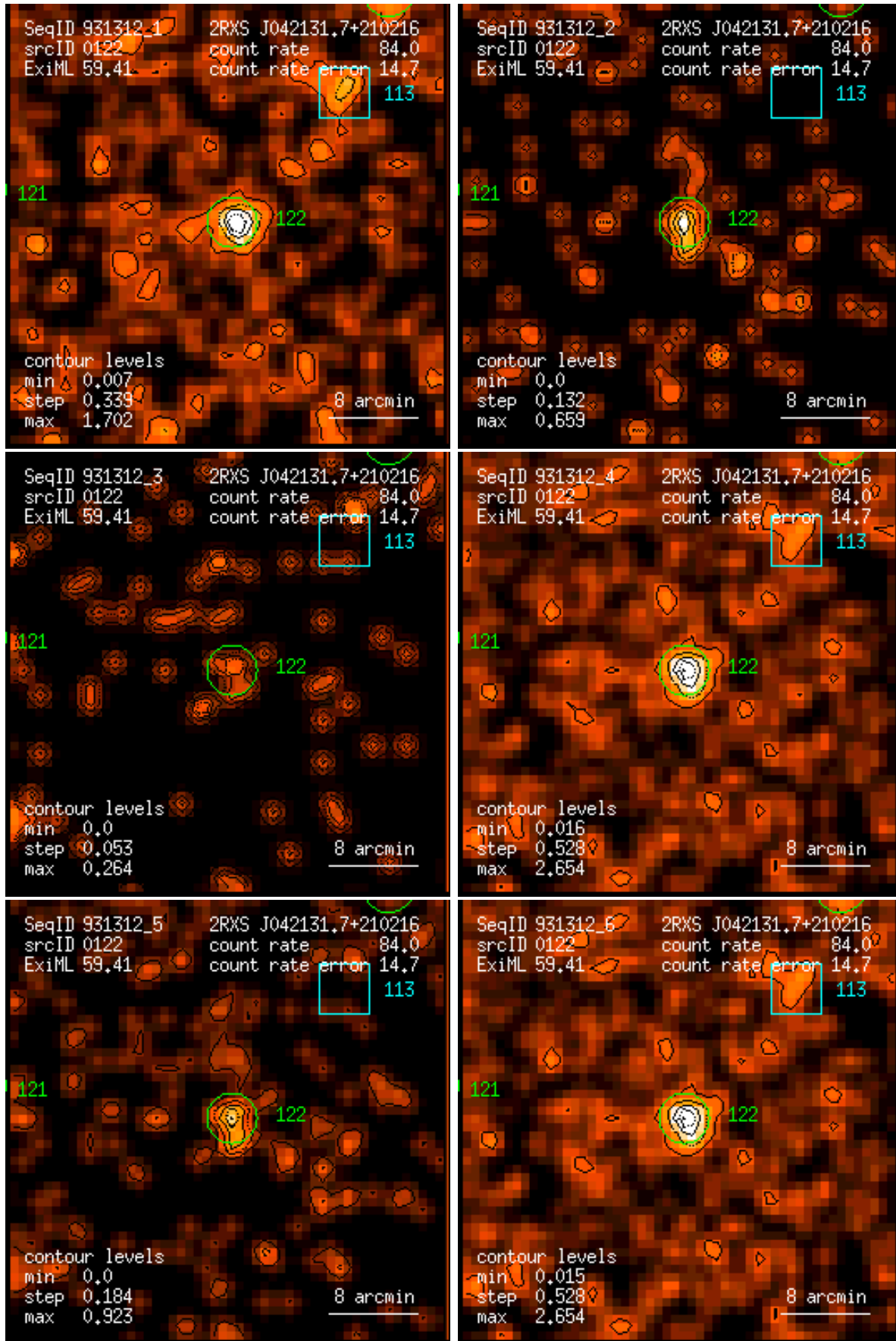
Figure 122: RASS 931312: detection 0122: band rate images, Gaussian filter: (1) PSPC channels 11 – 41, (2) 52 – 90, (3) 91 – 201, (4) 11 – 235, (5) 52 – 201, (6) 11 – 201. Broad band rates in counts/ks. Band rate contour levels in counts/ks/arcmin 2 .
