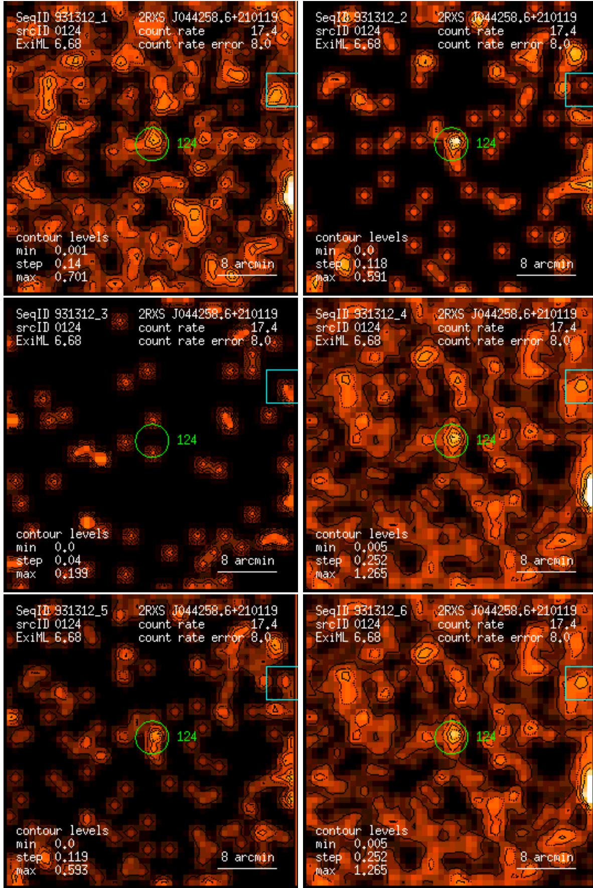
Figure 124: RASS 931312: detection 0124: band rate images, Gaussian filter: (1) PSPC channels 11 – 41, (2) 52 – 90, (3) 91 – 201, (4) 11 – 235, (5) 52 – 201, (6) 11 – 201. Broad band rates in counts/ks. Band rate contour levels in counts/ks/arcmin 2 .
