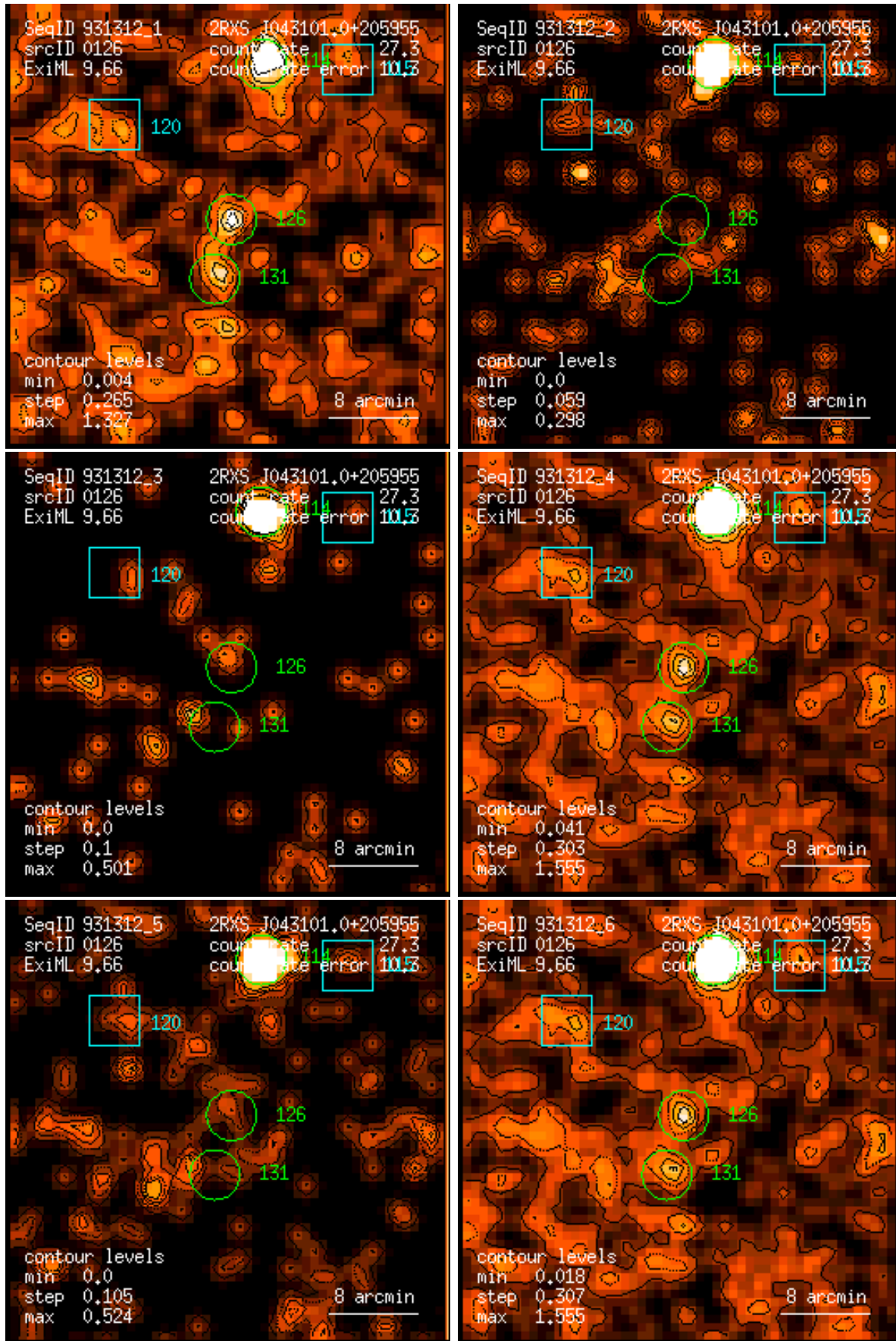
Figure 126: RASS 931312: detection 0126: band rate images, Gaussian filter: (1) PSPC channels 11 – 41, (2) 52 – 90, (3) 91 – 201, (4) 11 – 235, (5) 52 – 201, (6) 11 – 201. Broad band rates in counts/ks. Band rate contour levels in counts/ks/arcmin 2 .
