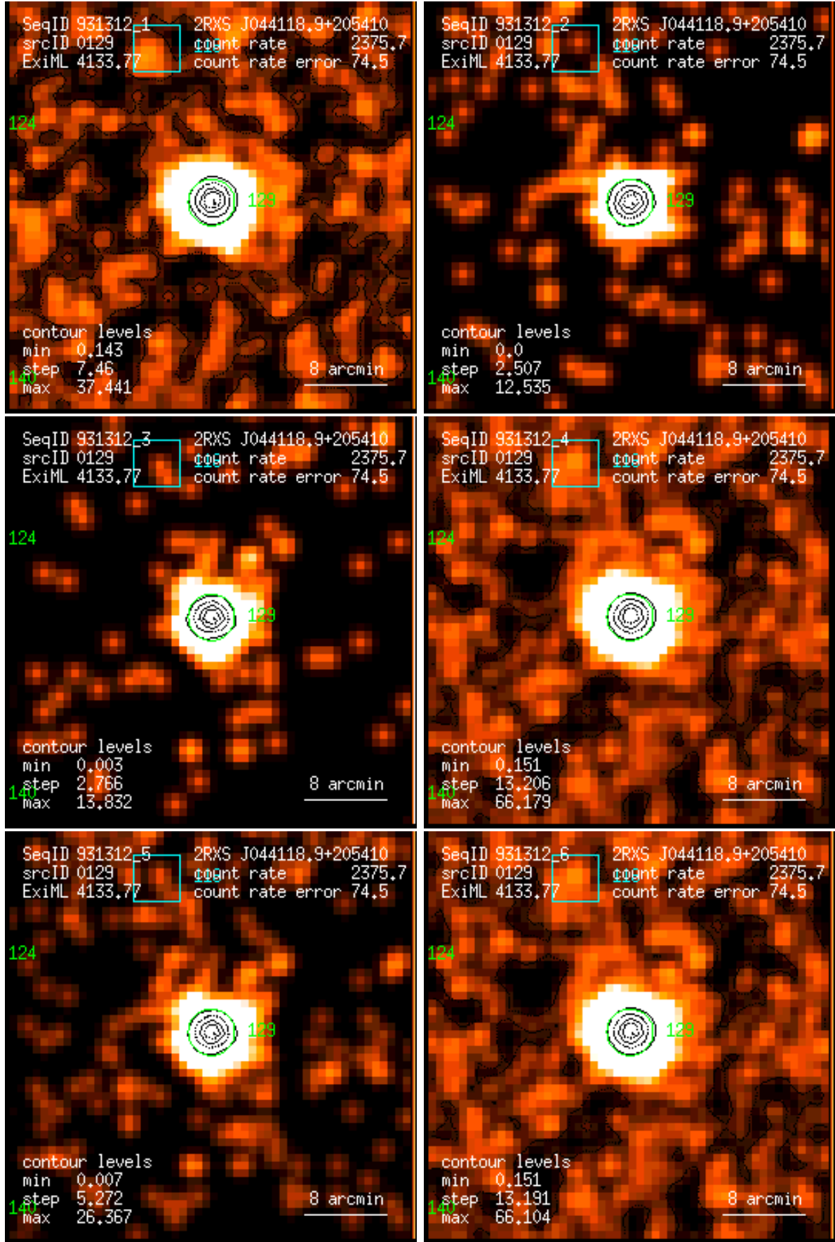
Figure 129: RASS 931312: detection 0129: band rate images, Gaussian filter: (1) PSPC channels 11 – 41, (2) 52 – 90, (3) 91 – 201, (4) 11 – 235, (5) 52 – 201, (6) 11 – 201. Broad band rates in counts/ks. Band rate contour levels in counts/ks/arcmin 2 .
