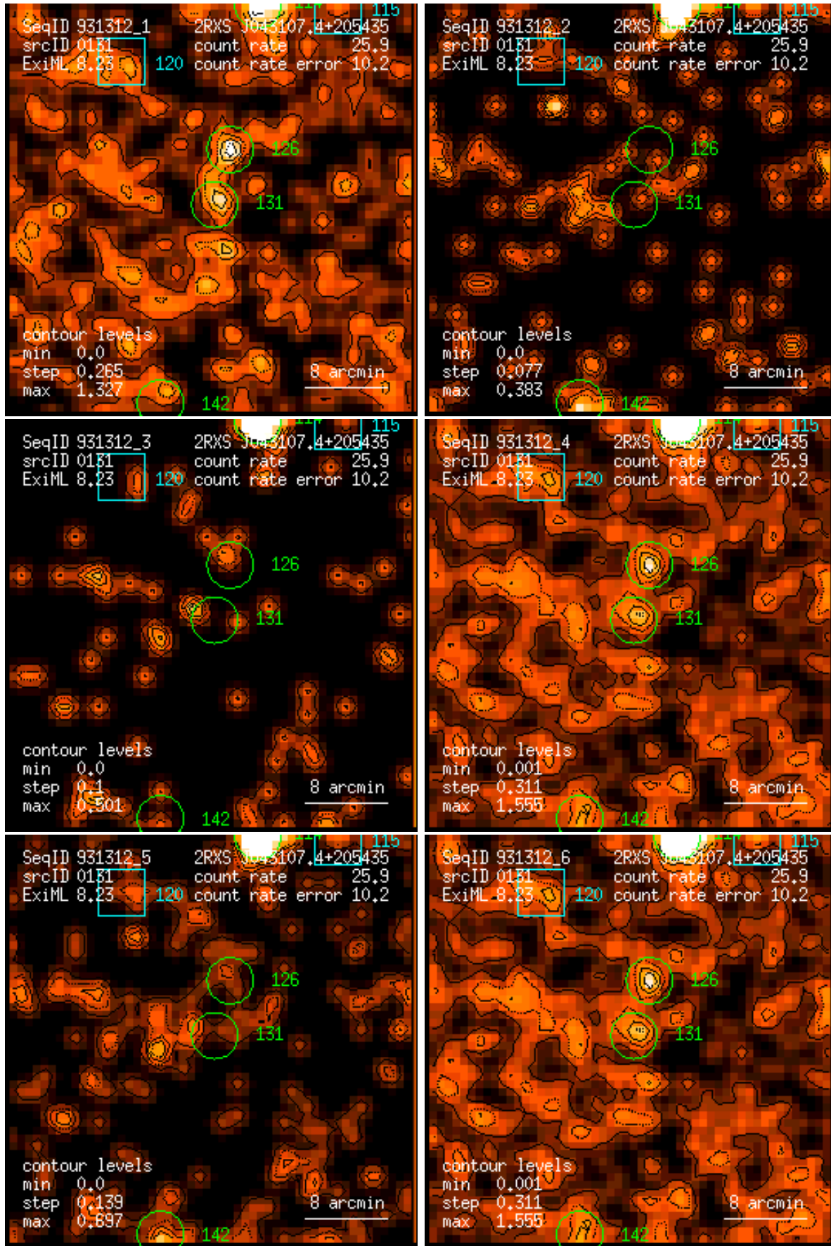
Figure 131: RASS 931312: detection 0131: band rate images, Gaussian filter: (1) PSPC channels 11 – 41, (2) 52 – 90, (3) 91 – 201, (4) 11 – 235, (5) 52 – 201, (6) 11 – 201. Broad band rates in counts/ks. Band rate contour levels in counts/ks/arcmin 2 .
