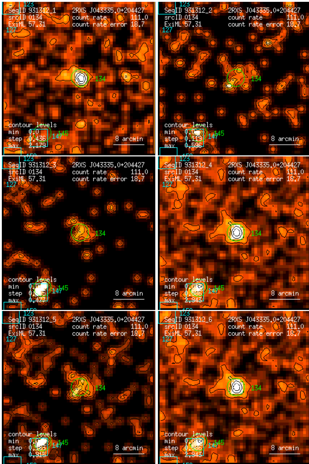
Figure 134: RASS 931312: detection 0134: band rate images, Gaussian filter: (1) PSPC channels 11 – 41, (2) 52 – 90, (3) 91 – 201, (4) 11 – 235, (5) 52 – 201, (6) 11 – 201. Broad band rates in counts/ks. Band rate contour levels in counts/ks/arcmin 2 .
