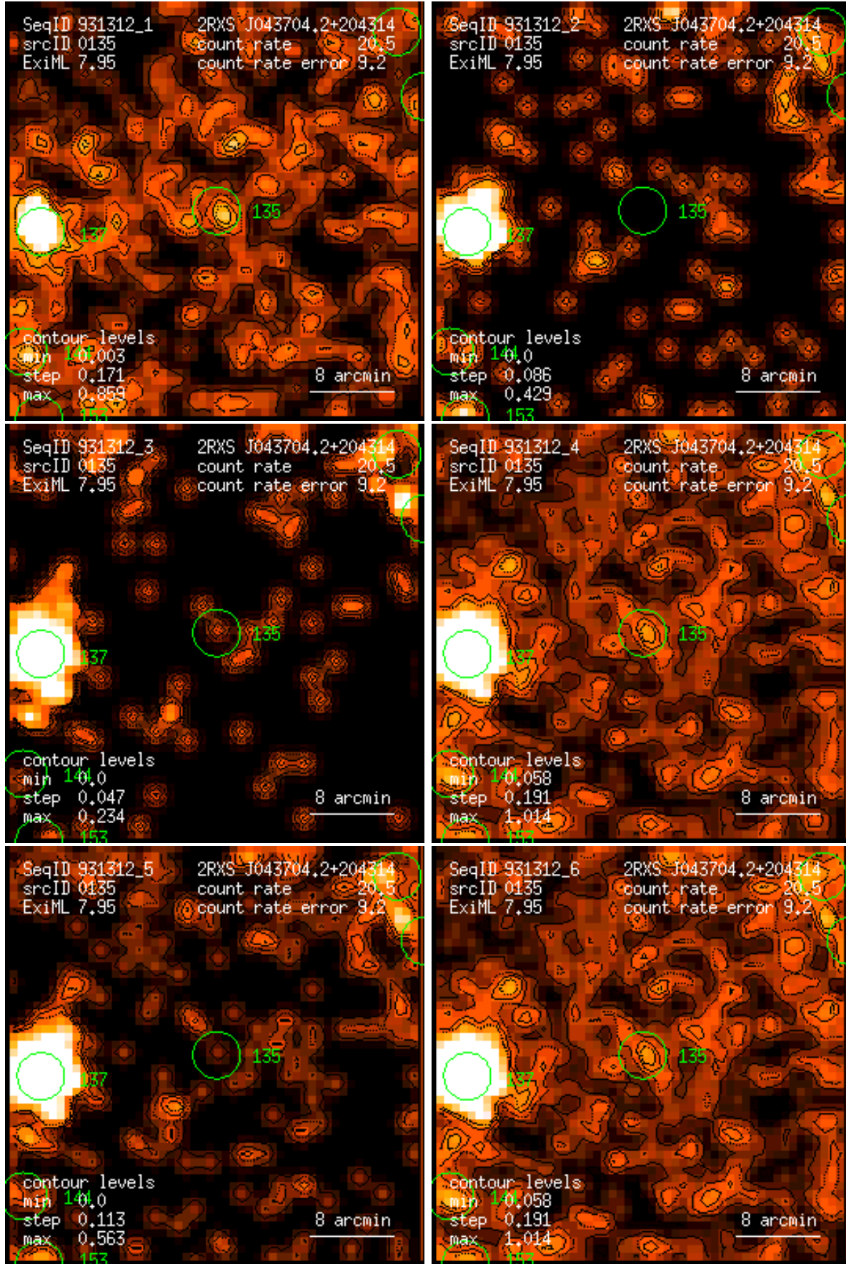
Figure 135: RASS 931312: detection 0135: band rate images, Gaussian filter: (1) PSPC channels 11 – 41, (2) 52 – 90, (3) 91 – 201, (4) 11 – 235, (5) 52 – 201, (6) 11 – 201. Broad band rates in counts/ks. Band rate contour levels in counts/ks/arcmin 2 .
