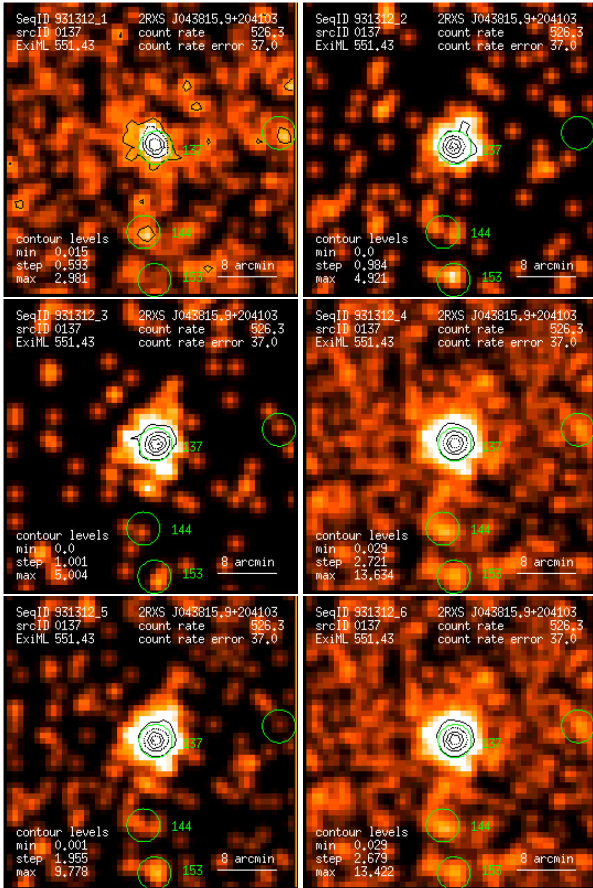
Figure 137: RASS 931312: detection 0137: band rate images, Gaussian filter: (1) PSPC channels 11 – 41, (2) 52 – 90, (3) 91 – 201, (4) 11 – 235, (5) 52 – 201, (6) 11 – 201. Broad band rates in counts/ks. Band rate contour levels in counts/ks/arcmin 2 .
