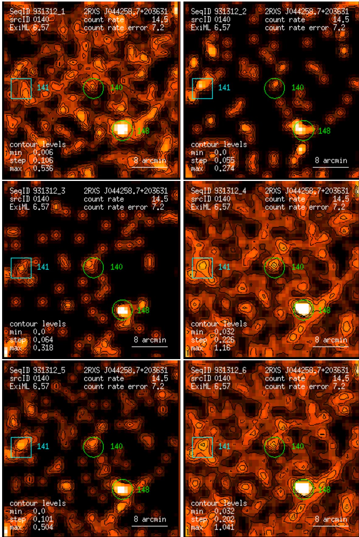
Figure 140: RASS 931312: detection 0140: band rate images, Gaussian filter: (1) PSPC channels 11 – 41, (2) 52 – 90, (3) 91 – 201, (4) 11 – 235, (5) 52 – 201, (6) 11 – 201. Broad band rates in counts/ks. Band rate contour levels in counts/ks/arcmin 2 .
