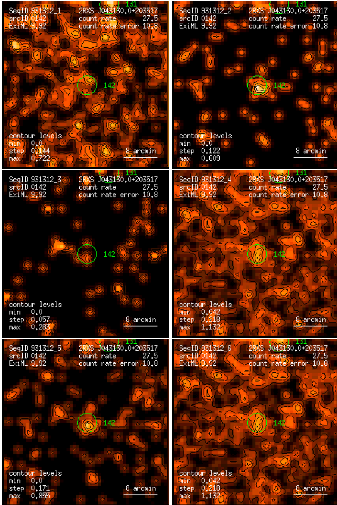
Figure 142: RASS 931312: detection 0142: band rate images, Gaussian filter: (1) PSPC channels 11 – 41, (2) 52 – 90, (3) 91 – 201, (4) 11 – 235, (5) 52 – 201, (6) 11 – 201. Broad band rates in counts/ks. Band rate contour levels in counts/ks/arcmin 2 .
