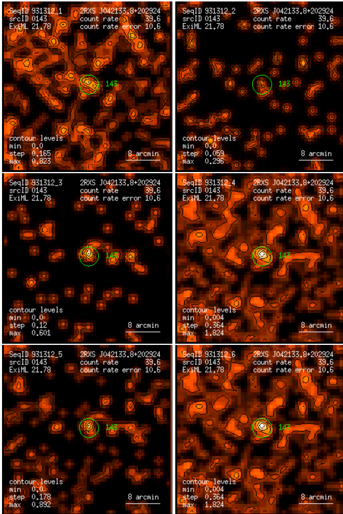
Figure 143: RASS 931312: detection 0143: band rate images, Gaussian filter: (1) PSPC channels 11 – 41, (2) 52 – 90, (3) 91 – 201, (4) 11 – 235, (5) 52 – 201, (6) 11 – 201. Broad band rates in counts/ks. Band rate contour levels in counts/ks/arcmin 2 .
