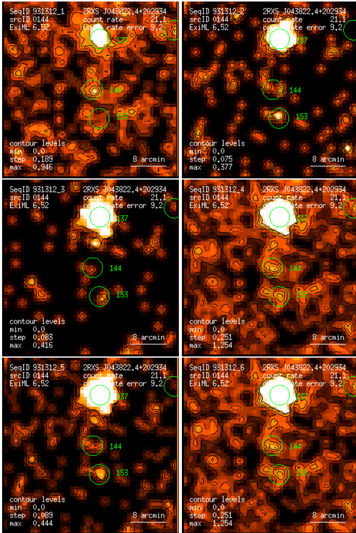
Figure 144: RASS 931312: detection 0144: band rate images, Gaussian filter: (1) PSPC channels 11 – 41, (2) 52 – 90, (3) 91 – 201, (4) 11 – 235, (5) 52 – 201, (6) 11 – 201. Broad band rates in counts/ks. Band rate contour levels in counts/ks/arcmin 2 .
