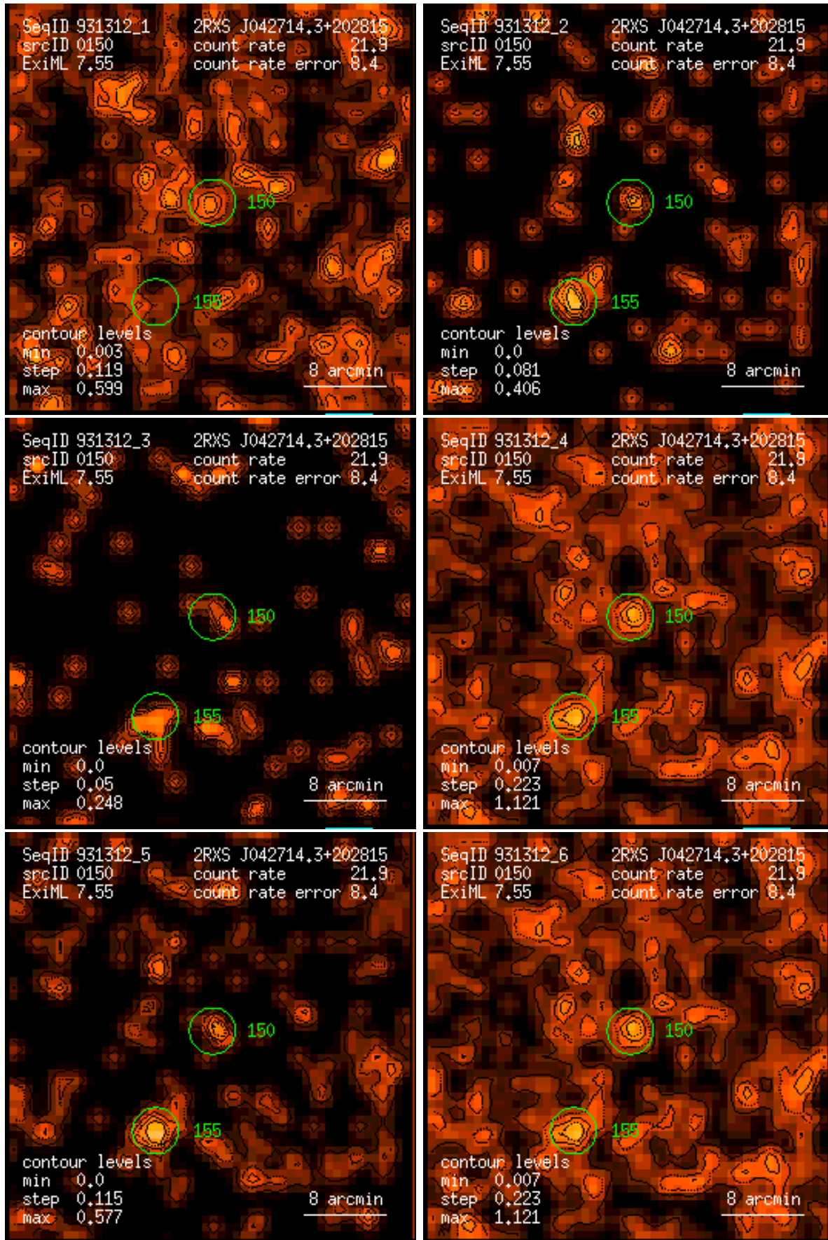
Figure 150: RASS 931312: detection 0150: band rate images, Gaussian filter: (1) PSPC channels 11 – 41, (2) 52 – 90, (3) 91 – 201, (4) 11 – 235, (5) 52 – 201, (6) 11 – 201. Broad band rates in counts/ks. Band rate contour levels in counts/ks/arcmin 2 .
