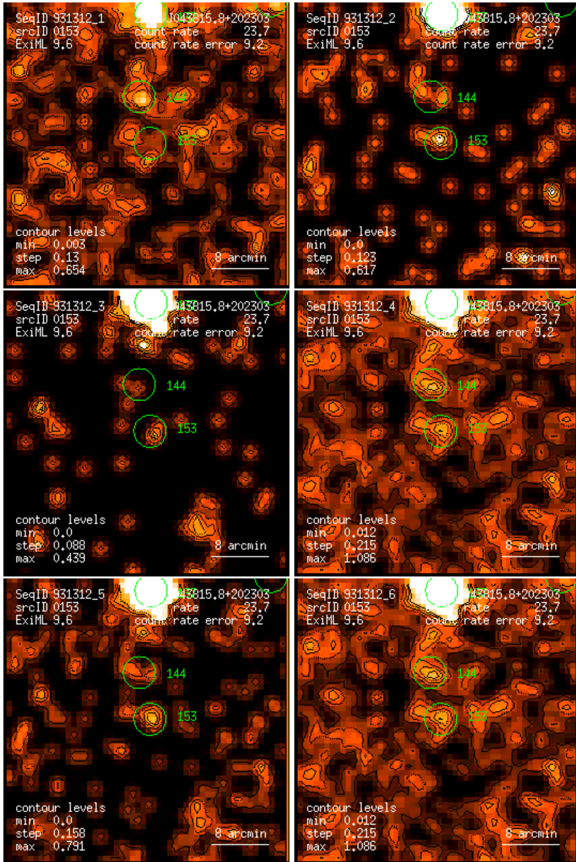
Figure 153: RASS 931312: detection 0153: band rate images, Gaussian filter: (1) PSPC channels 11 – 41, (2) 52 – 90, (3) 91 – 201, (4) 11 – 235, (5) 52 – 201, (6) 11 – 201. Broad band rates in counts/ks. Band rate contour levels in counts/ks/arcmin 2 .
