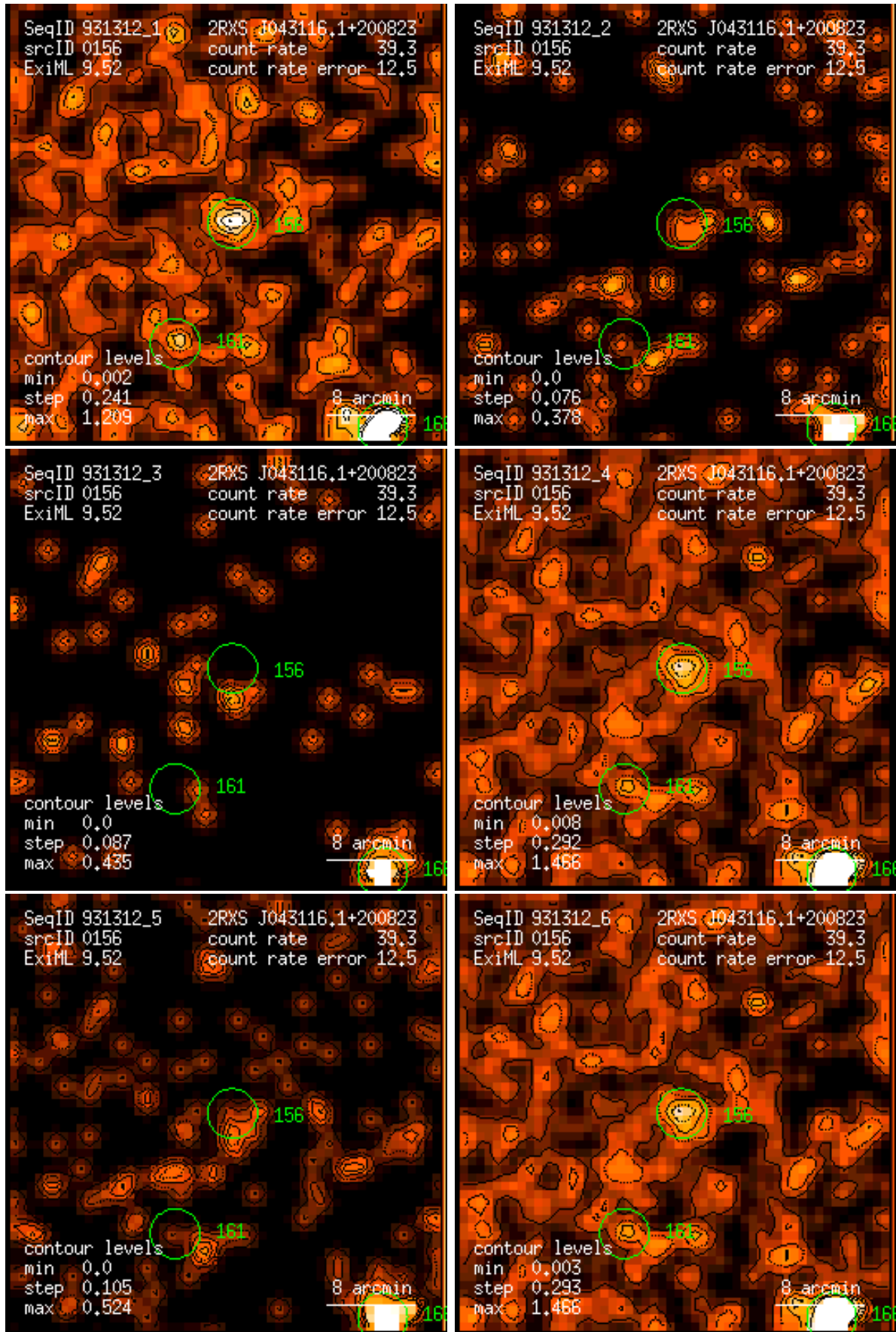
Figure 156: RASS 931312: detection 0156: band rate images, Gaussian filter: (1) PSPC channels 11 – 41, (2) 52 – 90, (3) 91 – 201, (4) 11 – 235, (5) 52 – 201, (6) 11 – 201. Broad band rates in counts/ks. Band rate contour levels in counts/ks/arcmin 2 .
