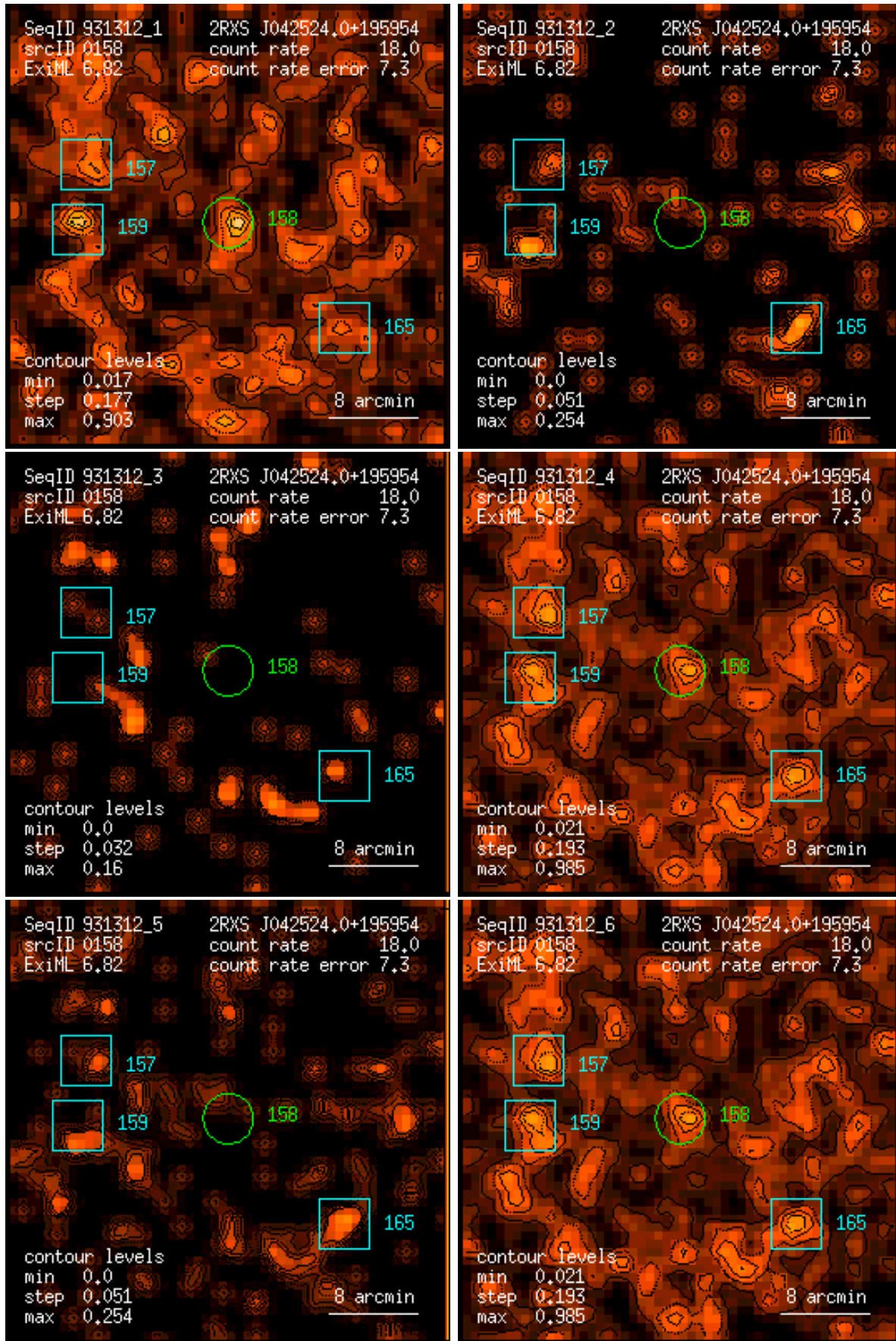
Figure 158: RASS 931312: detection 0158: band rate images, Gaussian filter: (1) PSPC channels 11 – 41, (2) 52 – 90, (3) 91 – 201, (4) 11 – 235, (5) 52 – 201, (6) 11 – 201. Broad band rates in counts/ks. Band rate contour levels in counts/ks/arcmin 2 .
