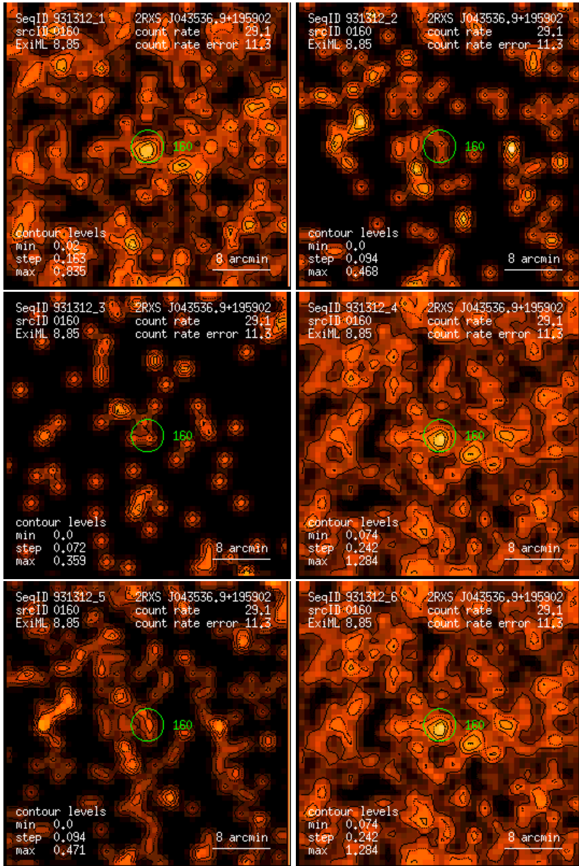
Figure 160: RASS 931312: detection 0160: band rate images, Gaussian filter: (1) PSPC channels 11 – 41, (2) 52 – 90, (3) 91 – 201, (4) 11 – 235, (5) 52 – 201, (6) 11 – 201. Broad band rates in counts/ks. Band rate contour levels in counts/ks/arcmin 2 .
