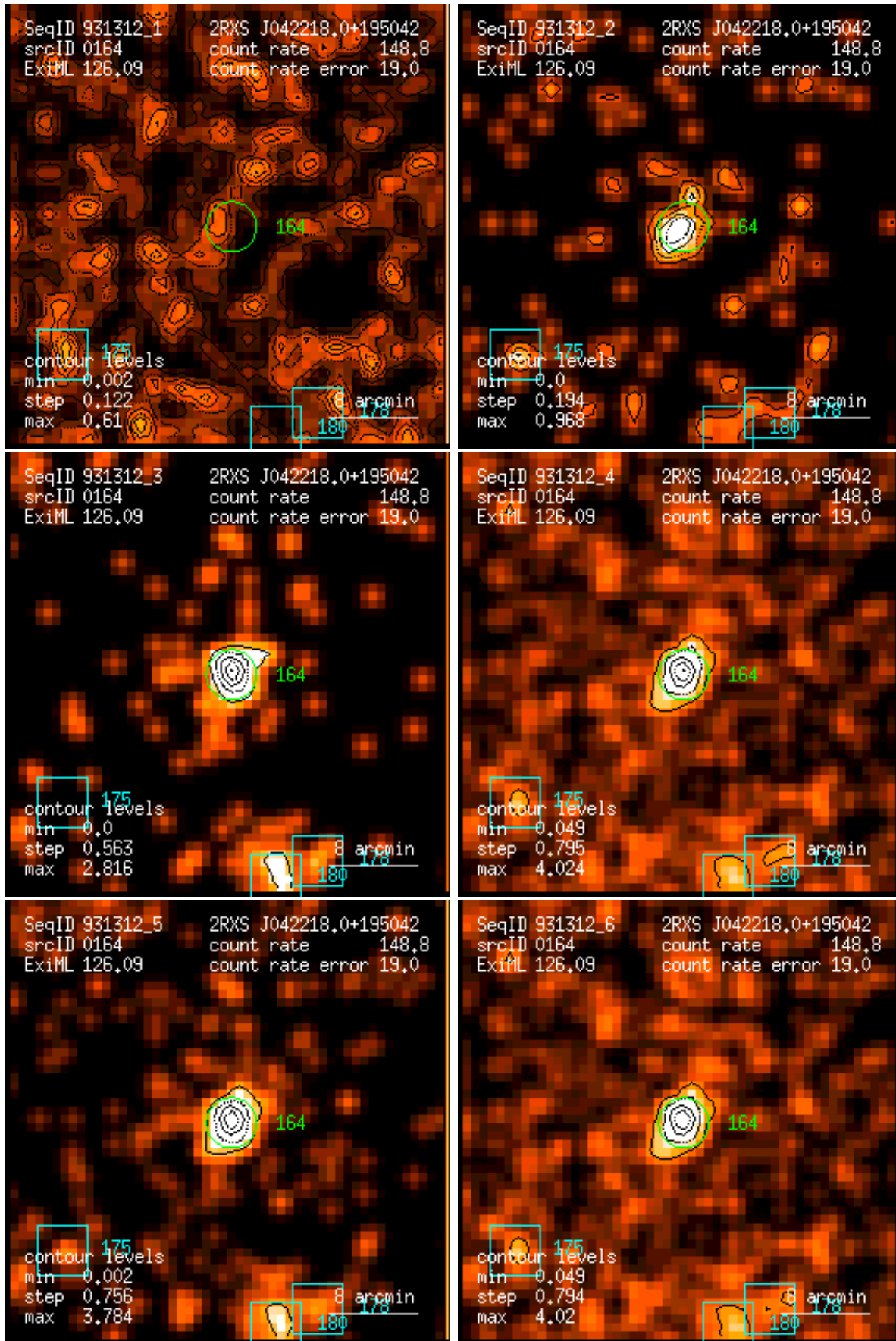
Figure 164: RASS 931312: detection 0164: band rate images, Gaussian filter: (1) PSPC channels 11 – 41, (2) 52 – 90, (3) 91 – 201, (4) 11 – 235, (5) 52 – 201, (6) 11 – 201. Broad band rates in counts/ks. Band rate contour levels in counts/ks/arcmin 2 .
