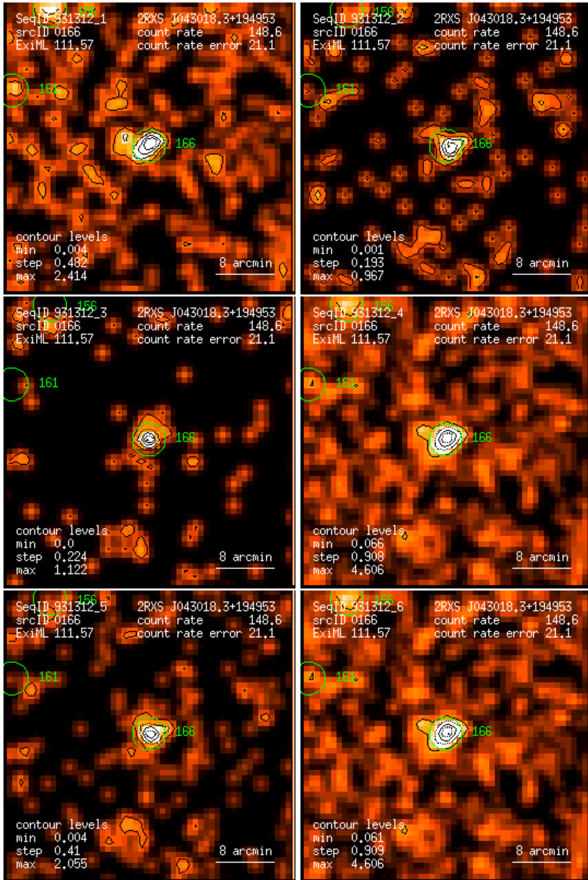
Figure 166: RASS 931312: detection 0166: band rate images, Gaussian filter: (1) PSPC channels 11 – 41, (2) 52 – 90, (3) 91 – 201, (4) 11 – 235, (5) 52 – 201, (6) 11 – 201. Broad band rates in counts/ks. Band rate contour levels in counts/ks/arcmin 2 .
