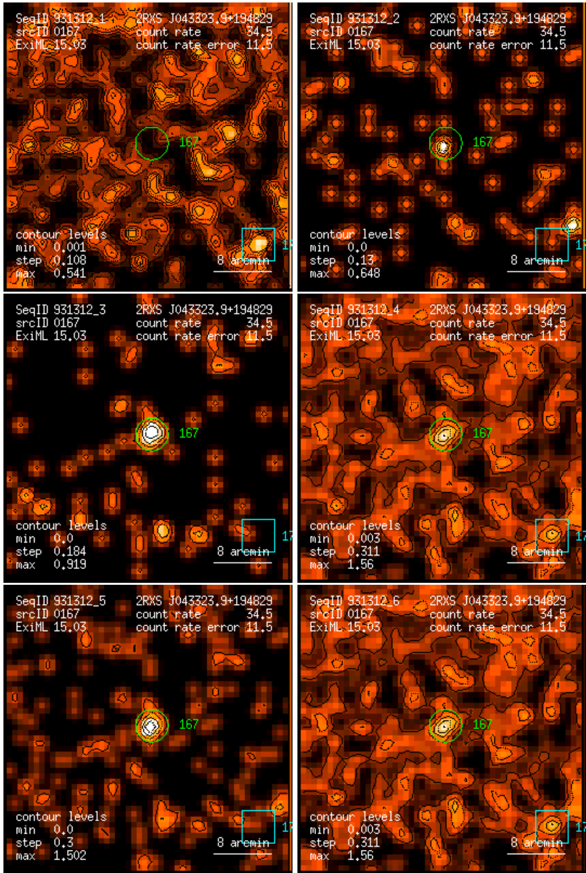
Figure 167: RASS 931312: detection 0167: band rate images, Gaussian filter: (1) PSPC channels 11 – 41, (2) 52 – 90, (3) 91 – 201, (4) 11 – 235, (5) 52 – 201, (6) 11 – 201. Broad band rates in counts/ks. Band rate contour levels in counts/ks/arcmin 2 .
