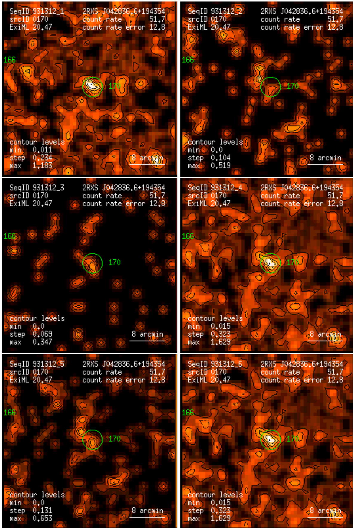
Figure 170: RASS 931312: detection 0170: band rate images, Gaussian filter: (1) PSPC channels 11 – 41, (2) 52 – 90, (3) 91 – 201, (4) 11 – 235, (5) 52 – 201, (6) 11 – 201. Broad band rates in counts/ks. Band rate contour levels in counts/ks/arcmin 2 .
