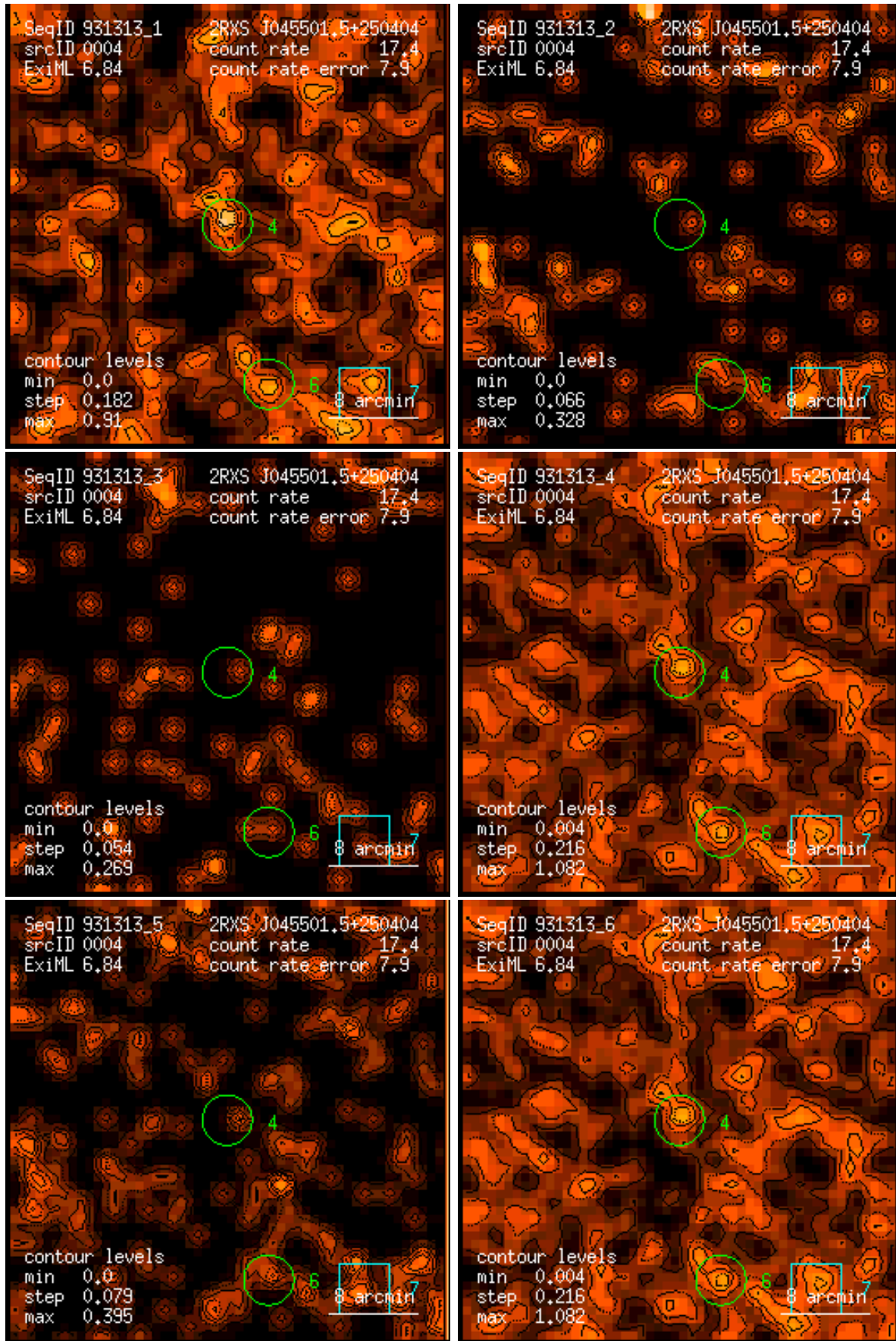
Figure 4: RASS 931313: detection 0004: band rate images, Gaussian filter: (1) PSPC channels 11 – 41, (2) 52 – 90, (3) 91 – 201, (4) 11 – 235, (5) 52 – 201, (6) 11 – 201. Broad band rates in counts/ks. Band rate contour levels in counts/ks/arcmin 2 .
