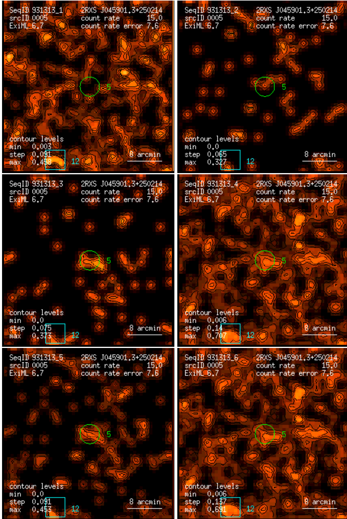
Figure 5: RASS 931313: detection 0005: band rate images, Gaussian filter: (1) PSPC channels 11 – 41, (2) 52 – 90, (3) 91 – 201, (4) 11 – 235, (5) 52 – 201, (6) 11 – 201. Broad band rates in counts/ks. Band rate contour levels in counts/ks/arcmin 2 .
