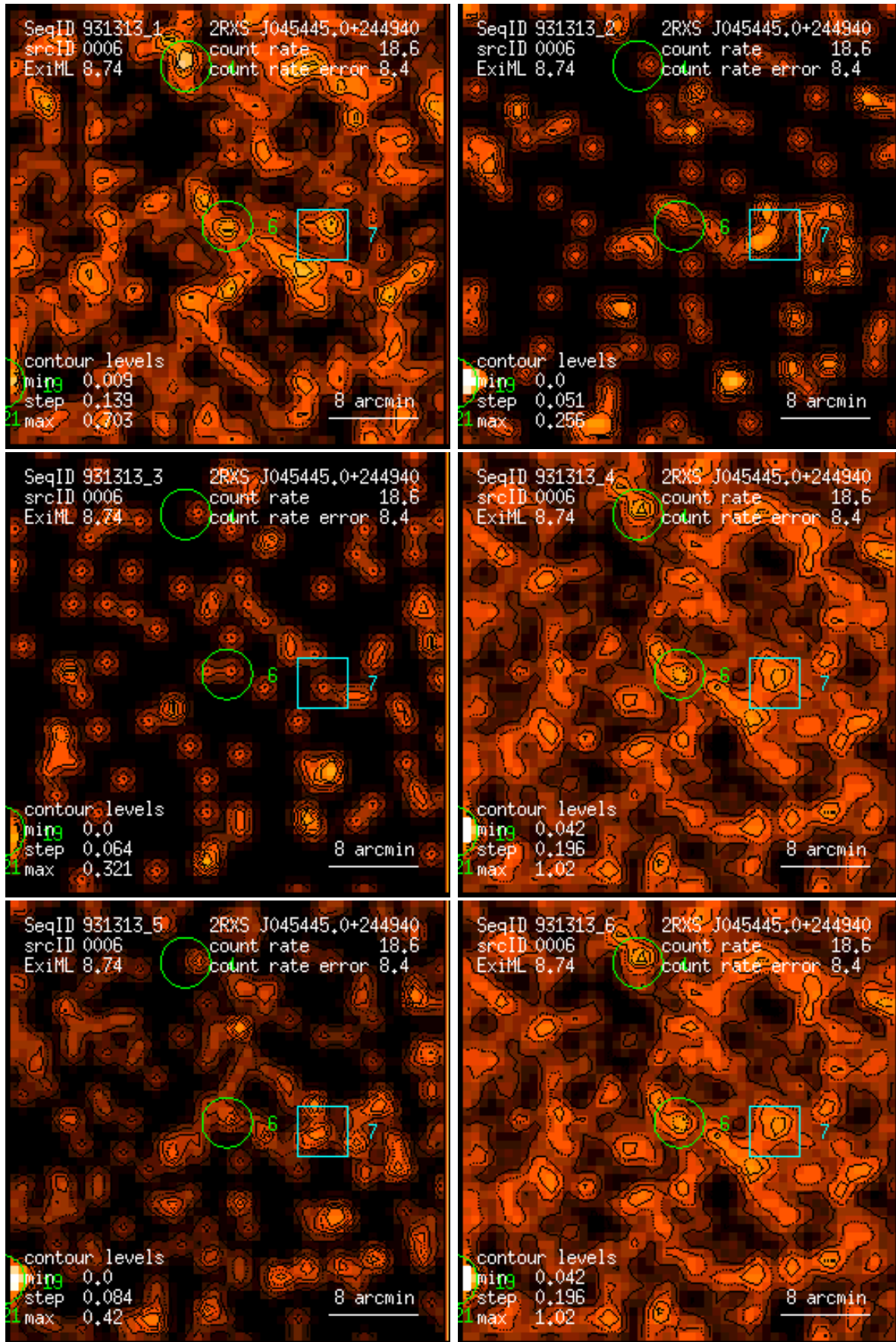
Figure 6: RASS 931313: detection 0006: band rate images, Gaussian filter: (1) PSPC channels 11 – 41, (2) 52 – 90, (3) 91 – 201, (4) 11 – 235, (5) 52 – 201, (6) 11 – 201. Broad band rates in counts/ks. Band rate contour levels in counts/ks/arcmin 2 .
