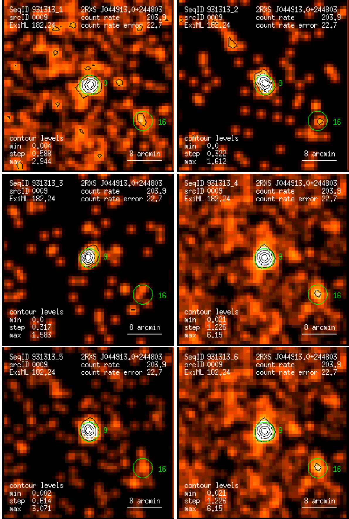
Figure 9: RASS 931313: detection 0009: band rate images, Gaussian filter: (1) PSPC channels 11 – 41, (2) 52 – 90, (3) 91 – 201, (4) 11 – 235, (5) 52 – 201, (6) 11 – 201. Broad band rates in counts/ks. Band rate contour levels in counts/ks/arcmin 2 .
