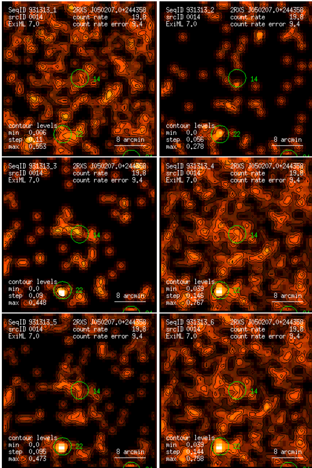
Figure 14: RASS 931313: detection 0014: band rate images, Gaussian filter: (1) PSPC channels 11 – 41, (2) 52 – 90, (3) 91 – 201, (4) 11 – 235, (5) 52 – 201, (6) 11 – 201. Broad band rates in counts/ks. Band rate contour levels in counts/ks/arcmin 2 .
