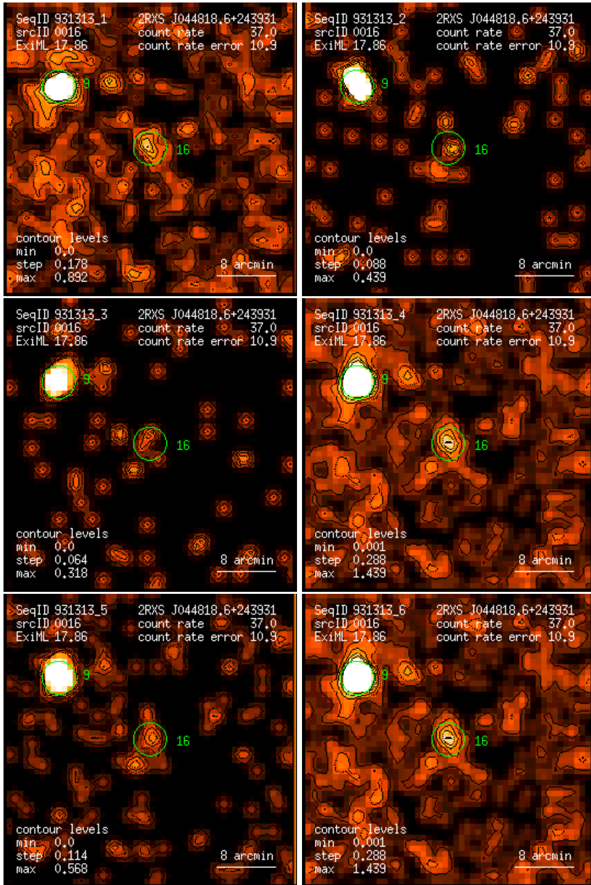
Figure 16: RASS 931313: detection 0016: band rate images, Gaussian filter: (1) PSPC channels 11 – 41, (2) 52 – 90, (3) 91 – 201, (4) 11 – 235, (5) 52 – 201, (6) 11 – 201. Broad band rates in counts/ks. Band rate contour levels in counts/ks/arcmin 2 .
