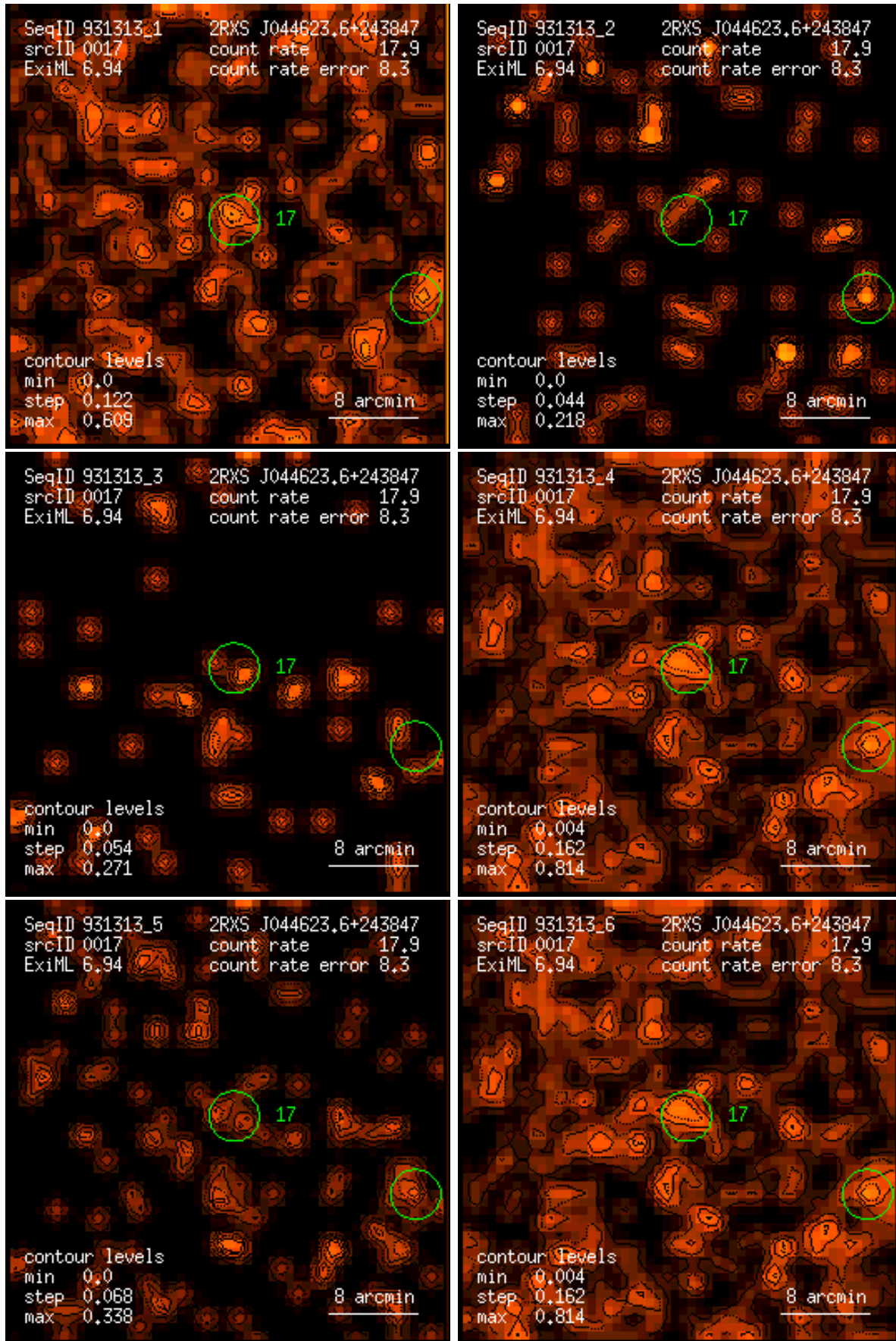
Figure 17: RASS 931313: detection 0017: band rate images, Gaussian filter: (1) PSPC channels 11 – 41, (2) 52 – 90, (3) 91 – 201, (4) 11 – 235, (5) 52 – 201, (6) 11 – 201. Broad band rates in counts/ks. Band rate contour levels in counts/ks/arcmin 2 .
