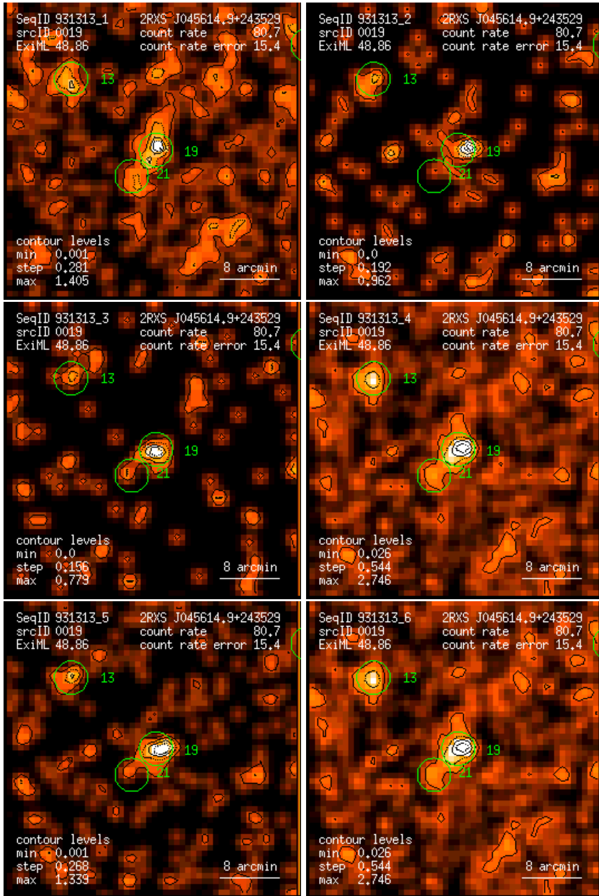
Figure 19: RASS 931313: detection 0019: band rate images, Gaussian filter: (1) PSPC channels 11 – 41, (2) 52 – 90, (3) 91 – 201, (4) 11 – 235, (5) 52 – 201, (6) 11 – 201. Broad band rates in counts/ks. Band rate contour levels in counts/ks/arcmin 2 .
