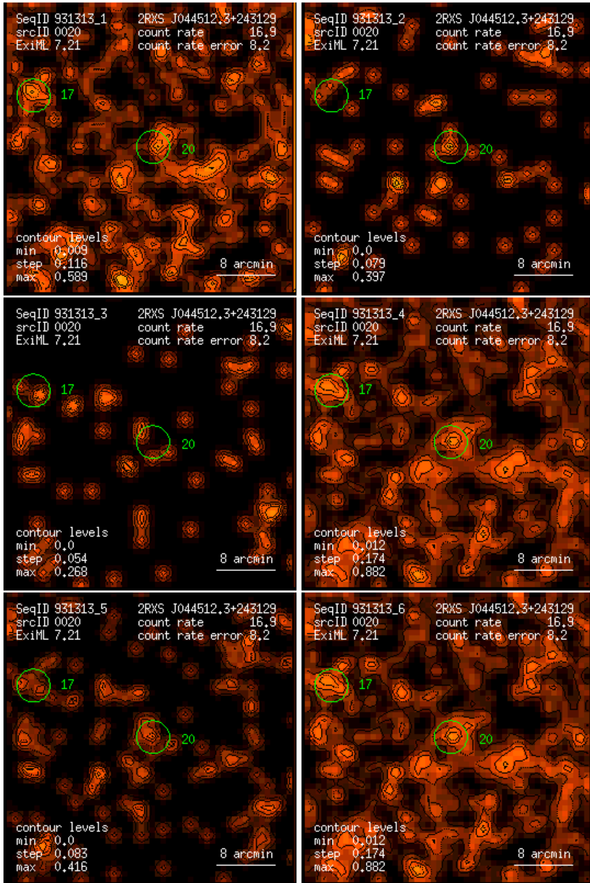
Figure 20: RASS 931313: detection 0020: band rate images, Gaussian filter: (1) PSPC channels 11 – 41, (2) 52 – 90, (3) 91 – 201, (4) 11 – 235, (5) 52 – 201, (6) 11 – 201. Broad band rates in counts/ks. Band rate contour levels in counts/ks/arcmin 2 .
