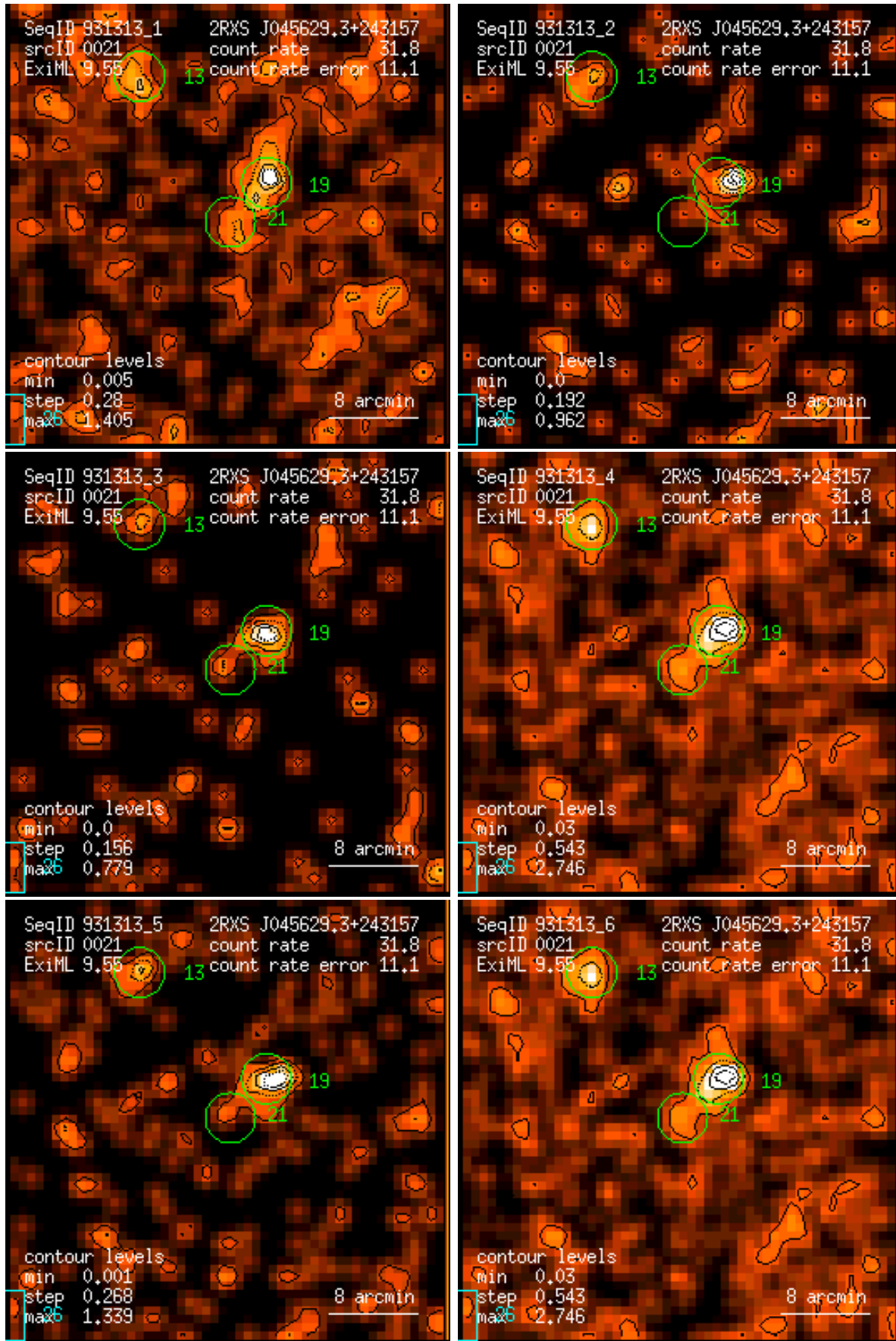
Figure 21: RASS 931313: detection 0021: band rate images, Gaussian filter: (1) PSPC channels 11 – 41, (2) 52 – 90, (3) 91 – 201, (4) 11 – 235, (5) 52 – 201, (6) 11 – 201. Broad band rates in counts/ks. Band rate contour levels in counts/ks/arcmin 2 .
