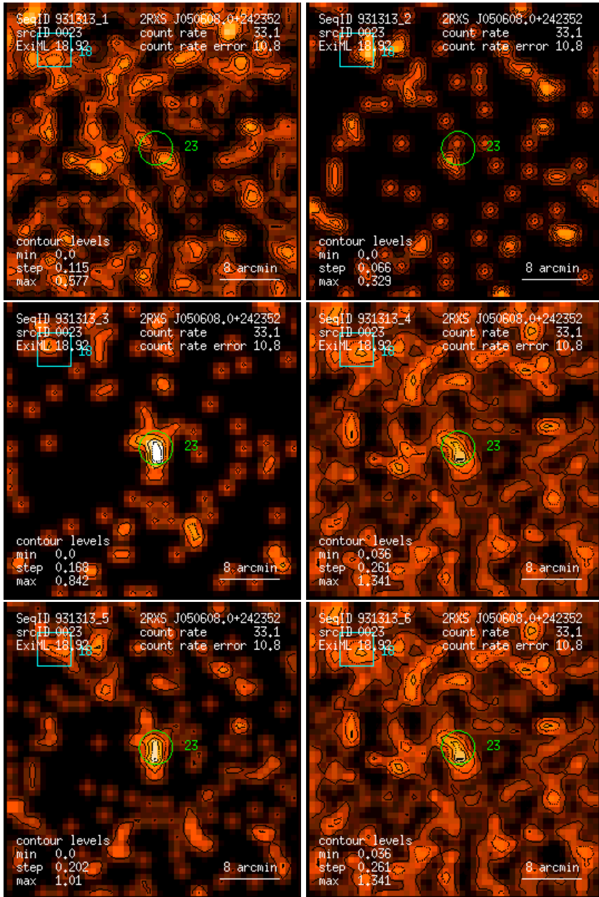
Figure 23: RASS 931313: detection 0023: band rate images, Gaussian filter: (1) PSPC channels 11 – 41, (2) 52 – 90, (3) 91 – 201, (4) 11 – 235, (5) 52 – 201, (6) 11 – 201. Broad band rates in counts/ks. Band rate contour levels in counts/ks/arcmin 2 .
