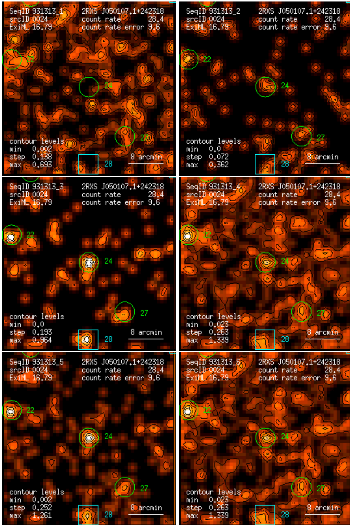
Figure 24: RASS 931313: detection 0024: band rate images, Gaussian filter: (1) PSPC channels 11 – 41, (2) 52 – 90, (3) 91 – 201, (4) 11 – 235, (5) 52 – 201, (6) 11 – 201. Broad band rates in counts/ks. Band rate contour levels in counts/ks/arcmin 2 .
