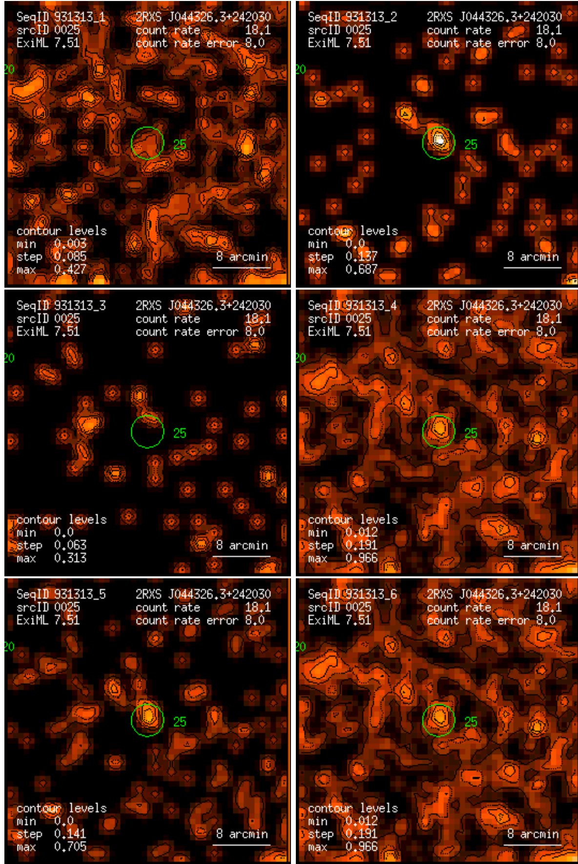
Figure 25: RASS 931313: detection 0025: band rate images, Gaussian filter: (1) PSPC channels 11 – 41, (2) 52 – 90, (3) 91 – 201, (4) 11 – 235, (5) 52 – 201, (6) 11 – 201. Broad band rates in counts/ks. Band rate contour levels in counts/ks/arcmin 2 .
