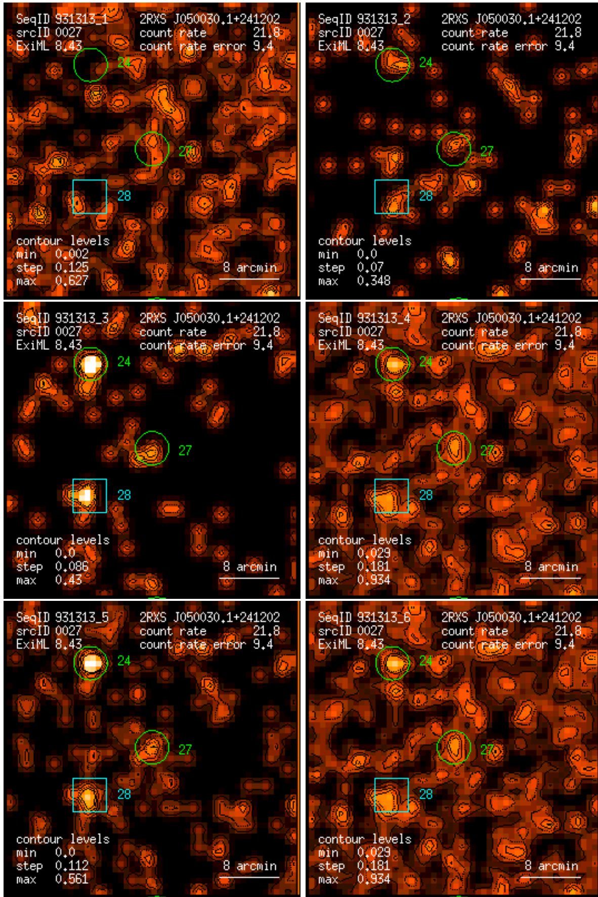
Figure 27: RASS 931313: detection 0027: band rate images, Gaussian filter: (1) PSPC channels 11 – 41, (2) 52 – 90, (3) 91 – 201, (4) 11 – 235, (5) 52 – 201, (6) 11 – 201. Broad band rates in counts/ks. Band rate contour levels in counts/ks/arcmin 2 .
