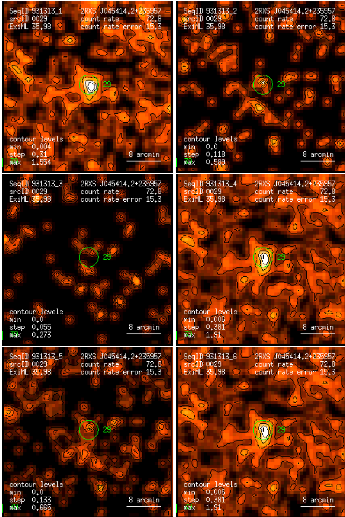
Figure 29: RASS 931313: detection 0029: band rate images, Gaussian filter: (1) PSPC channels 11 – 41, (2) 52 – 90, (3) 91 – 201, (4) 11 – 235, (5) 52 – 201, (6) 11 – 201. Broad band rates in counts/ks. Band rate contour levels in counts/ks/arcmin 2 .
