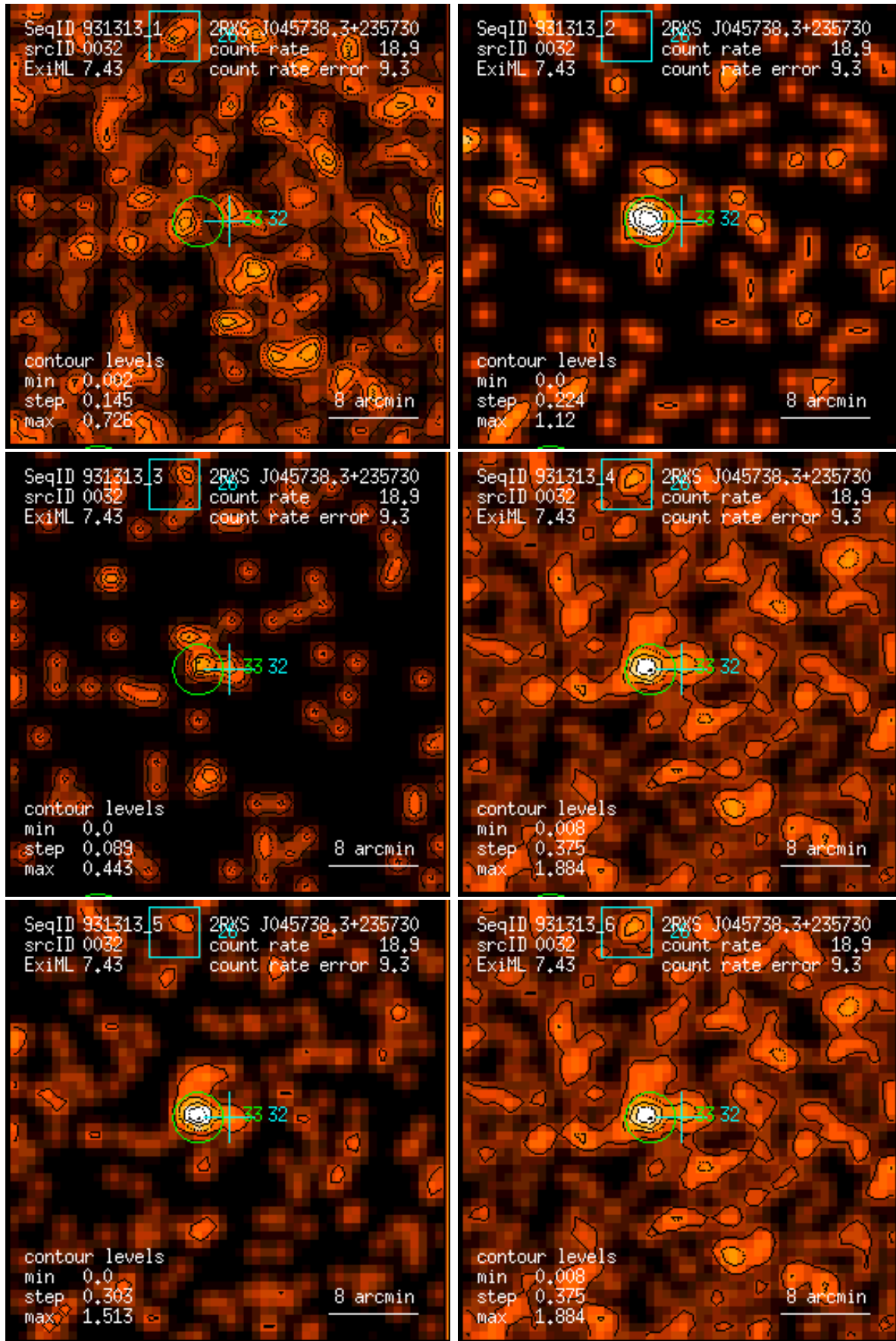
Figure 32: RASS 931313: detection 0032: band rate images, Gaussian filter: (1) PSPC channels 11 – 41, (2) 52 – 90, (3) 91 – 201, (4) 11 – 235, (5) 52 – 201, (6) 11 – 201. Broad band rates in counts/ks. Band rate contour levels in counts/ks/arcmin 2 .
