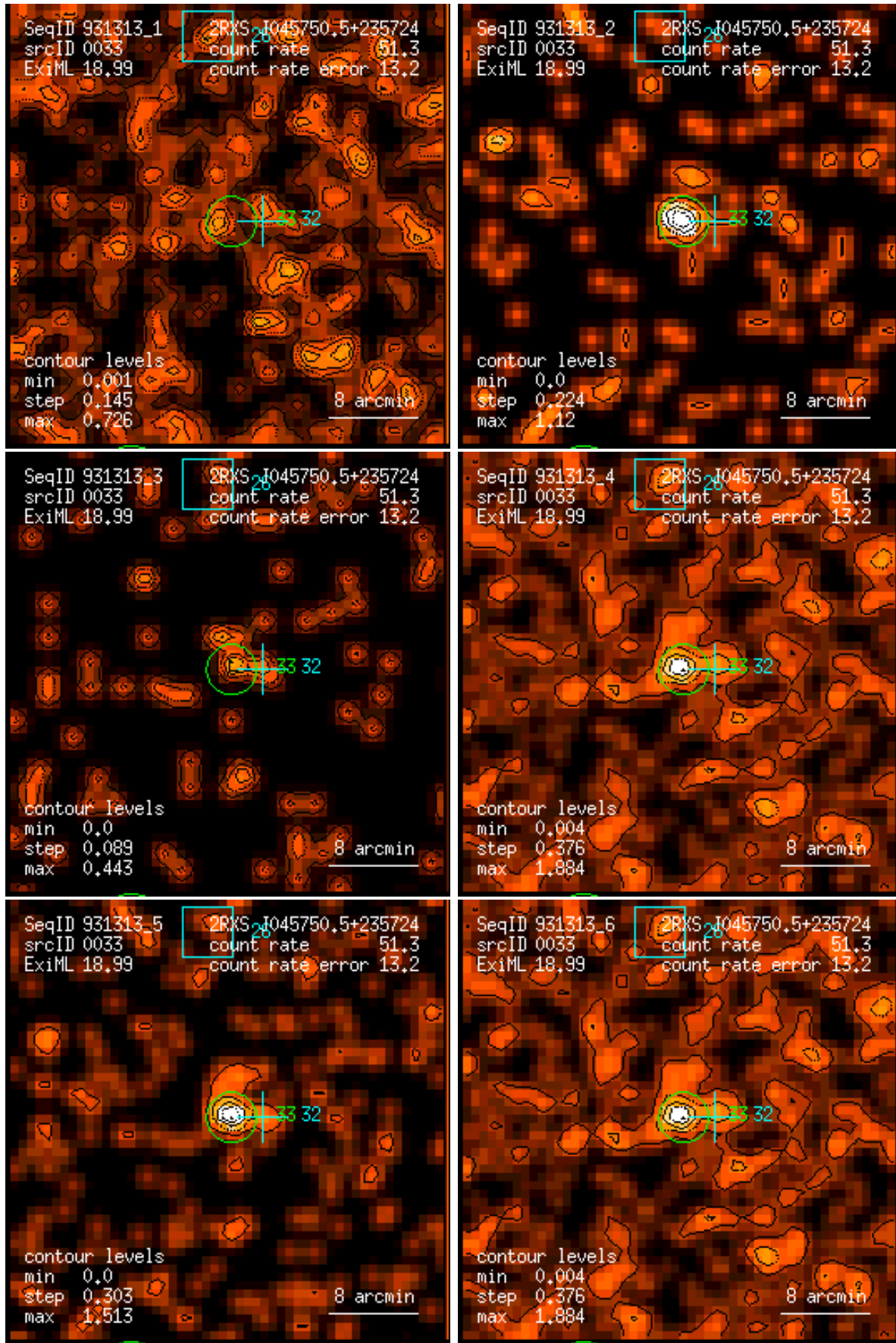
Figure 33: RASS 931313: detection 0033: band rate images, Gaussian filter: (1) PSPC channels 11 – 41, (2) 52 – 90, (3) 91 – 201, (4) 11 – 235, (5) 52 – 201, (6) 11 – 201. Broad band rates in counts/ks. Band rate contour levels in counts/ks/arcmin 2 .
