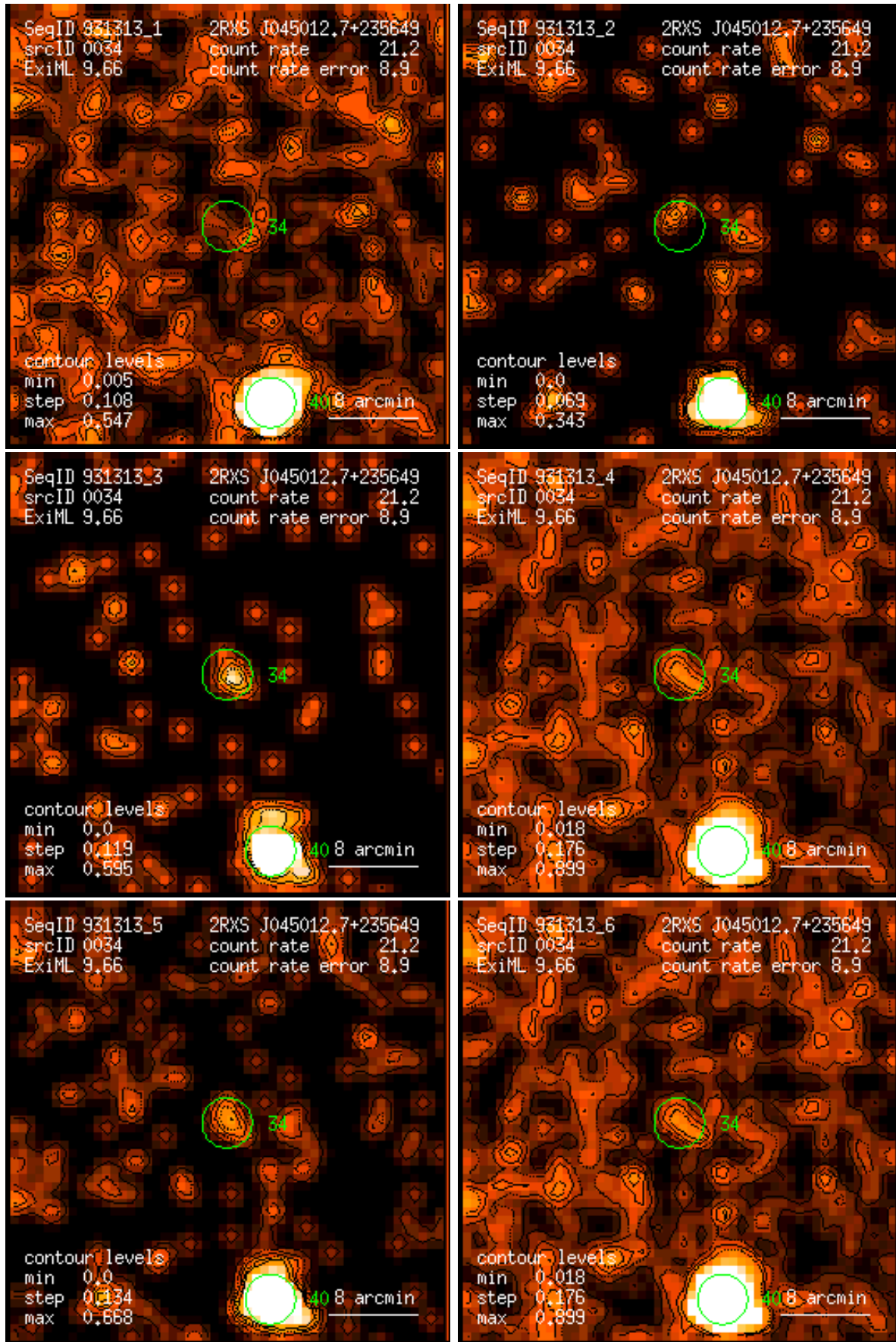
Figure 34: RASS 931313: detection 0034: band rate images, Gaussian filter: (1) PSPC channels 11 – 41, (2) 52 – 90, (3) 91 – 201, (4) 11 – 235, (5) 52 – 201, (6) 11 – 201. Broad band rates in counts/ks. Band rate contour levels in counts/ks/arcmin 2 .
