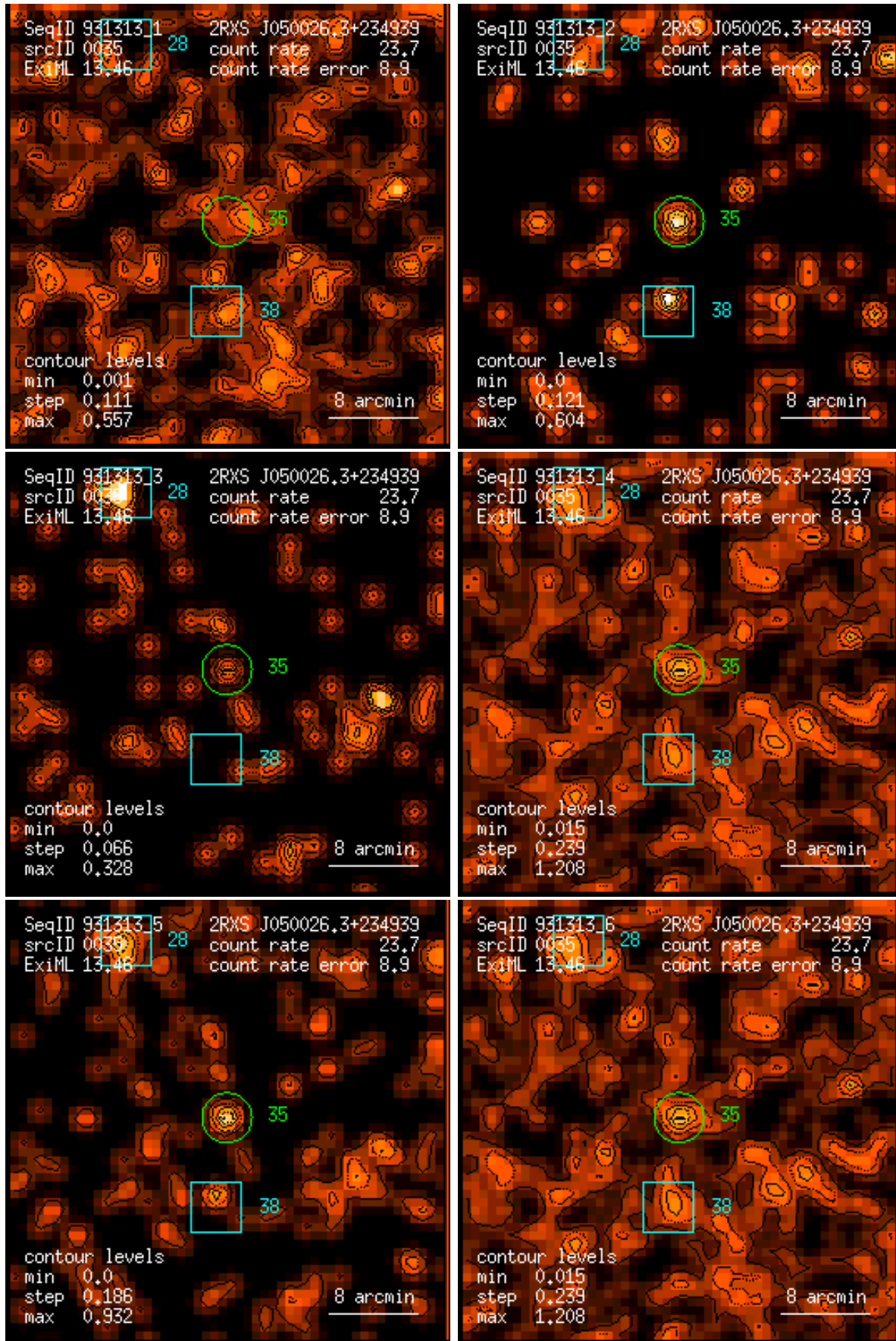
Figure 35: RASS 931313: detection 0035: band rate images, Gaussian filter: (1) PSPC channels 11 – 41, (2) 52 – 90, (3) 91 – 201, (4) 11 – 235, (5) 52 – 201, (6) 11 – 201. Broad band rates in counts/ks. Band rate contour levels in counts/ks/arcmin 2 .
